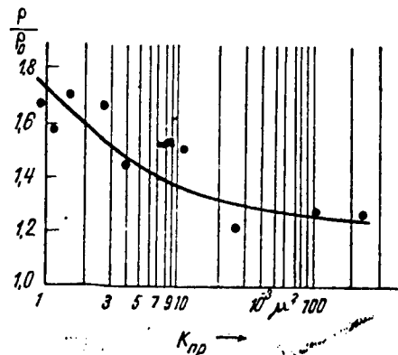
Figure 3. Relationship Between Permeability Coefficient K_{np} and Resistivity \rho/\rho_0 at an Effective Stress of 50 MPa for Tested Rock
