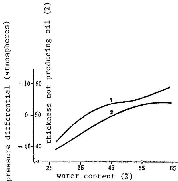
Figure 3. Reference graph from the Xing Bei area showing that pressure differential is not enough to overcome the relationship between water content and the thickness of the non-producing part of the stratum.
