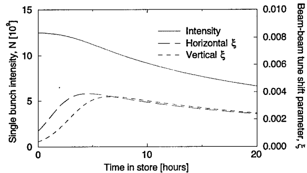
Figure 5: Beam-beam tune shift parameter evolution.
