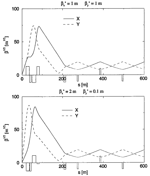
Figure 2: Round and flat ( \kappa = 0.05 ) IR optics, with a common magnet layout.
