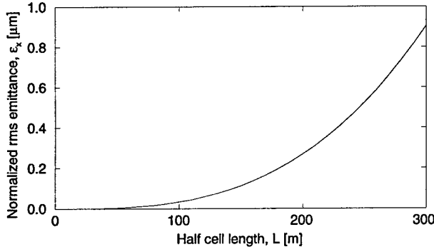
Figure 1: Equilibrium emittance versus half cell length
