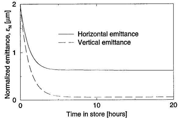
Figure 4: Emittance evolution, with radiation and IBS.
