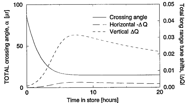
Figure 6: Long range tune shift evolution, per IR.
