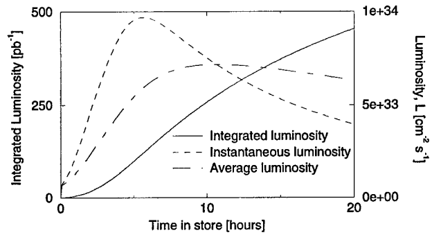
Figure 3: Luminosity evolution during a 20 hour store.
