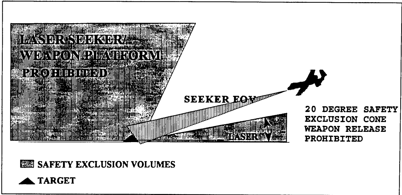
Figure 4-5. Sample side view of safety exclusion volumes for ground laser designator.
