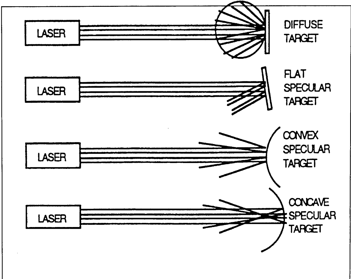
Figure 6-1. Diffuse reflection and specular reflection.
