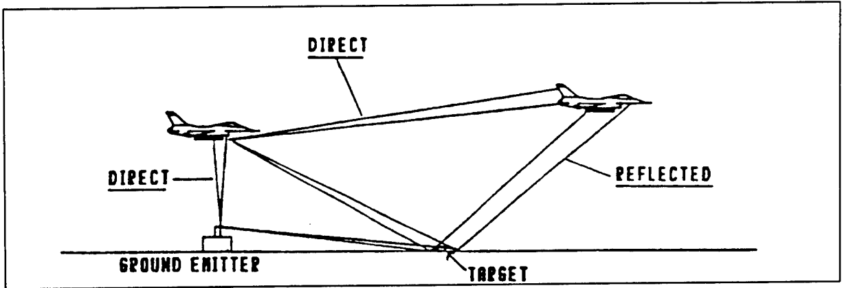
Figure E-14. Potential exposure modes.
