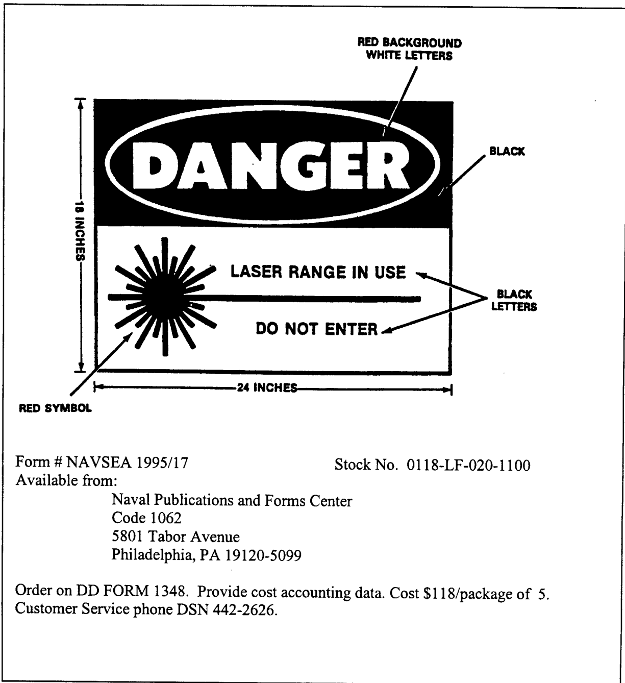
Figure 4-3. Example: warning sign.
