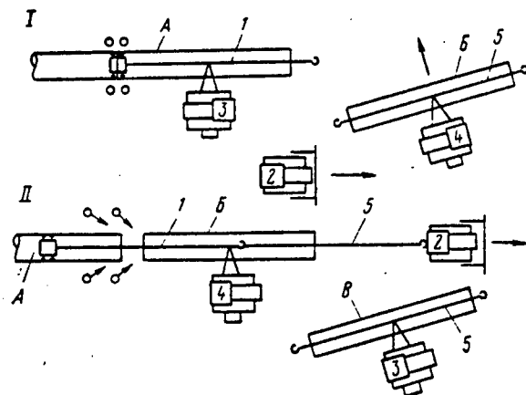
Figure 4. Scheme for Operating with a Centering Guide That Has a Long Separable Rod.
