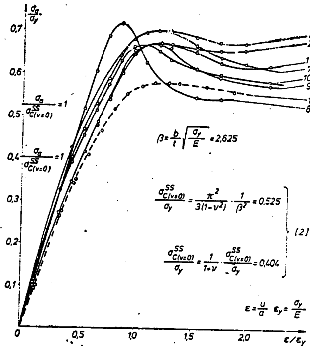
Fig. 4. Load carrying capacity of simply supported square and rectangular plates having very small initial deflections ( v = 0 )
