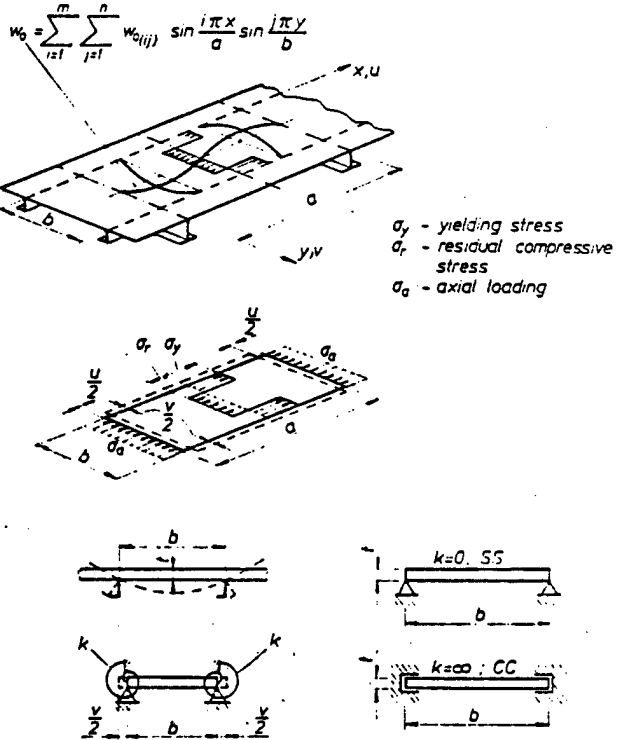
Fig. 1. Axially loaded plate having stresses and deflections and different boundary conditions
