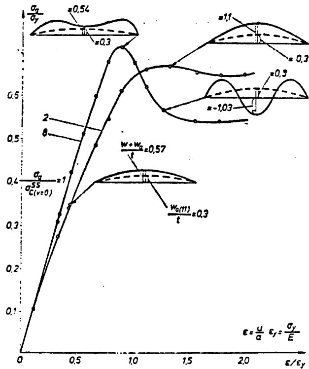
Fig. 6. Behaviour of square and rectangular simply supported plates having the same initial deflections ( \nu = 0 )
