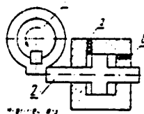
Fig. 13. Mechanism of angular positioning of the spindle of HP4: 1 - spindle, 2 - stopper lock (a - on, b - off)
