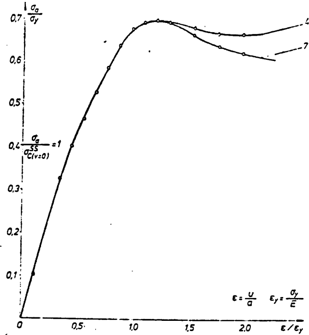
Fig. 5. Load carrying capacity of simply supported square and rectangular plates having very small initial deflections ( \nu = 0 )
