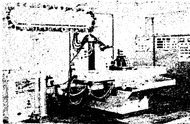
Fig. 2. Experimental prototype of horizontal machining center FXF 50NM
