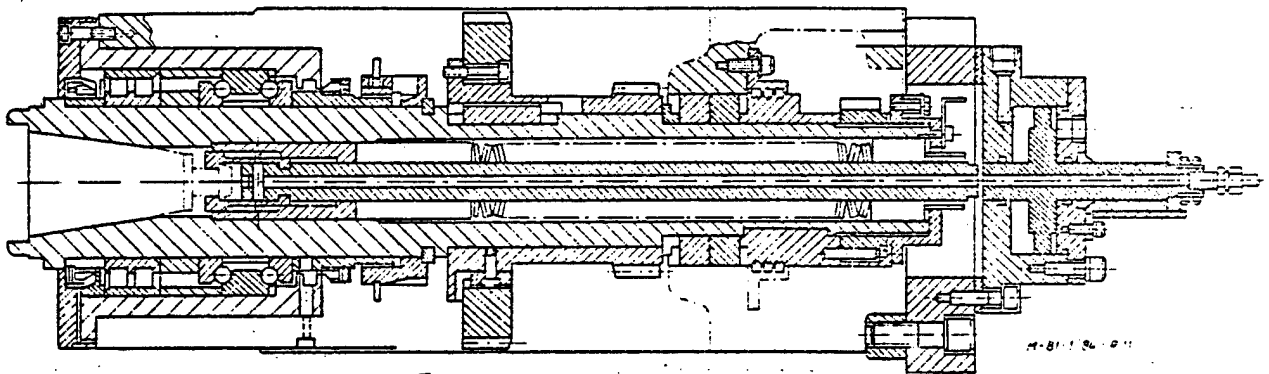
Fig. 11. Spindles of HP mounted on bearings
