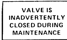
Figure IV-4. OR-Gate for Human Error
