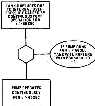
Figure VIII-5. Fault Tree Construction – Step 3
