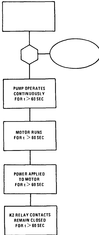
Figure VIII-6. Fault Tree Construction – Step 4
