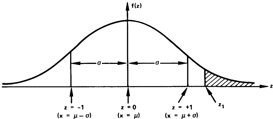
Figure X-7. The Standardized Normal Distribution
