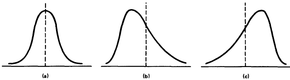
Figure X-3. Typical Shapes for f(x)
