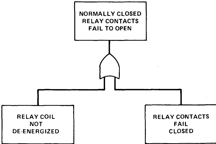
Figure VII-3. A Specific Two-Input OR-Gate
