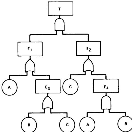
Figure VII-10. Example Fault Tree
