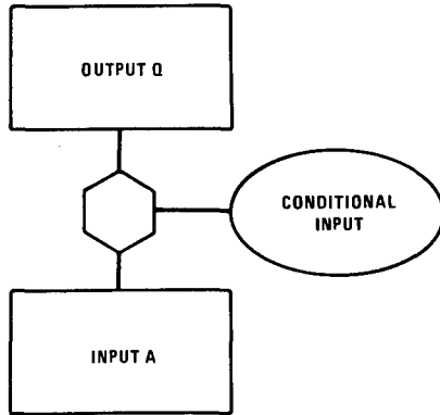
Figure IV-8. The INHIBIT-Gate
