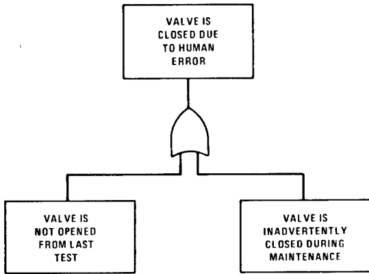
Figure IV-4. OR-Gate for Human Error
