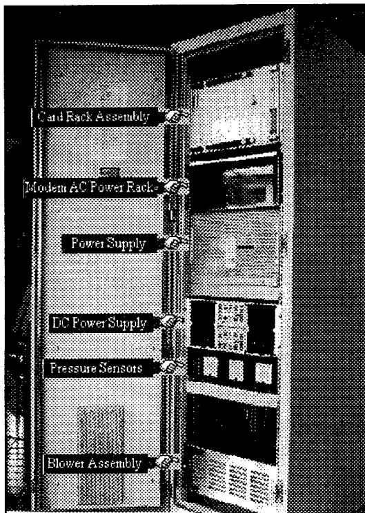
Figure 7. ASOS Pressure Sensor
