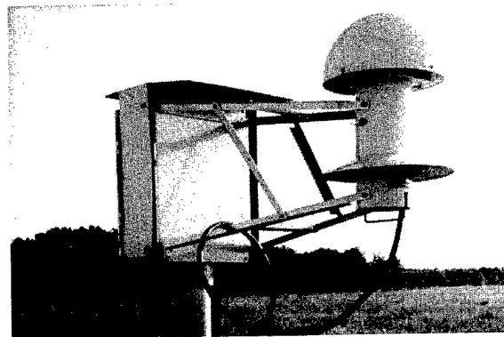
Figure 5. ASOS Hygrothermometer
