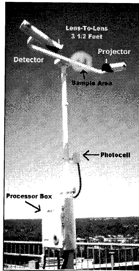
Figure 13. Forward Scatter Visibility Sensor
