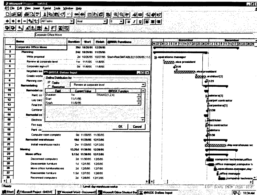
Figure K-3. @RISK for Microsoft Project: Specify a Random Variable
