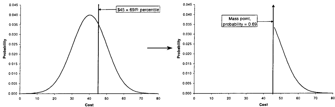
Figure III-4. Density Functions Before and After Transformation
