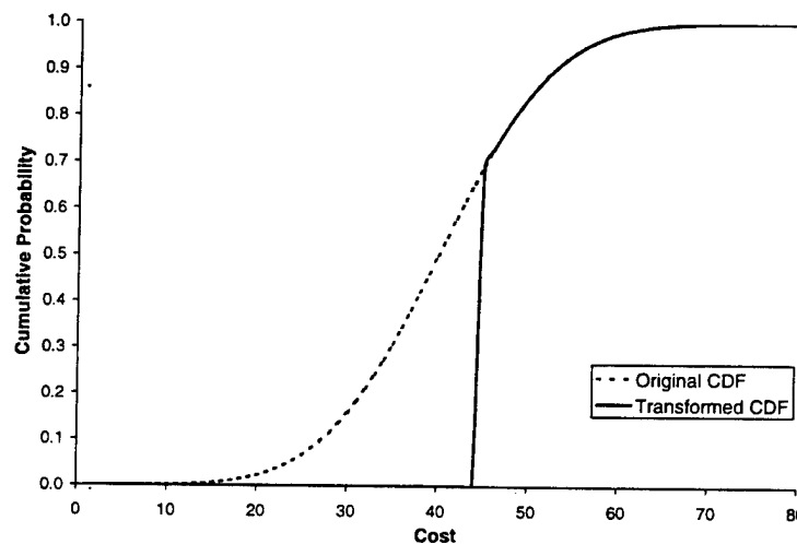
Figure III-5. Cumulative Distribution Functions Before and After Transformation
