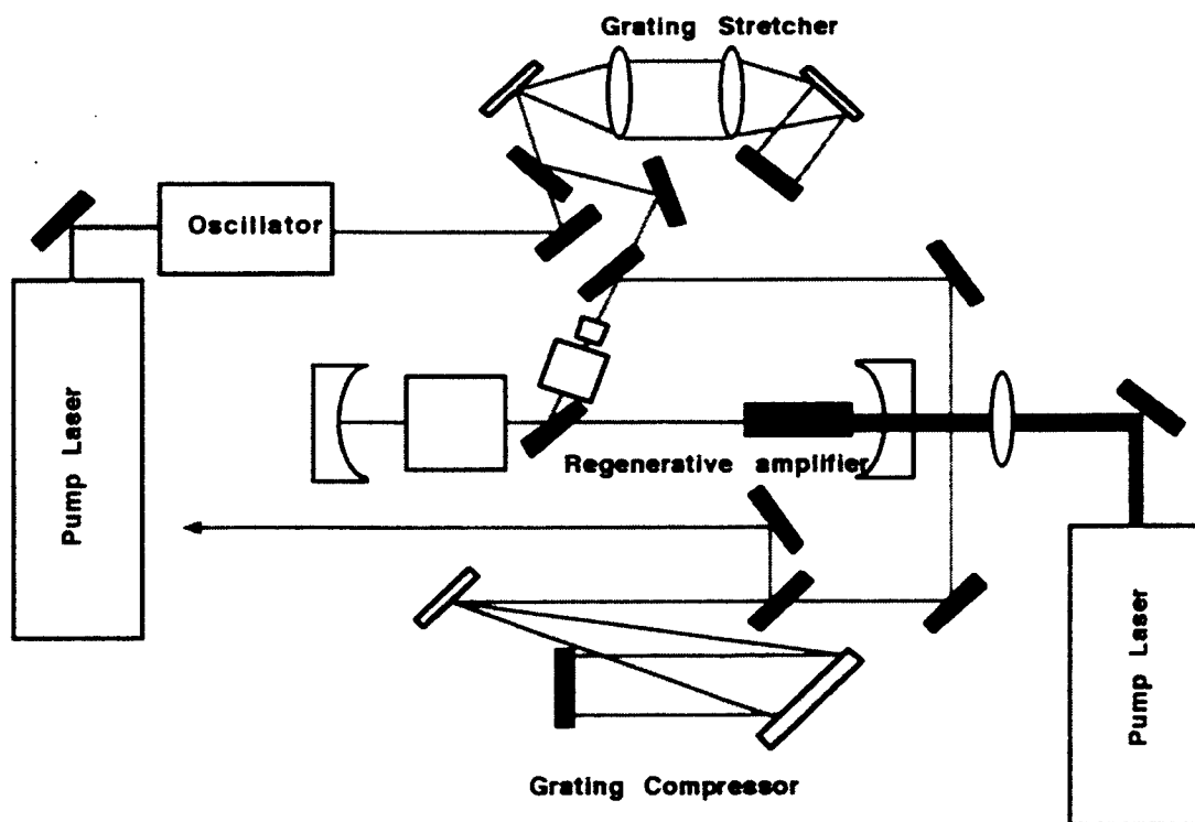
Figure 1. The kilohertz Ti:Sapphire system used in the experiments. A Ti:Sapphire oscillator produces the seed pulses which are stretched using a 1200 1/mm grating pair. The pulses are amplified to 1 mJ in the regenerative amplifier at kilohertz repetition rates. The pulses are recompressed by a 1200 1/mm grating pair which results in 50 fs, 500 \mu\text{J} pulses.
