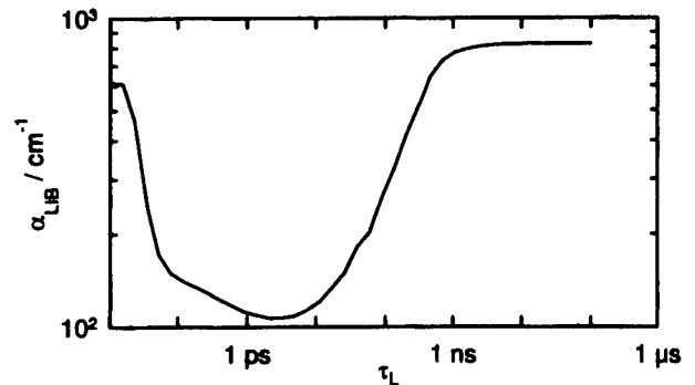
Figure 5: Calculated time averaged absorption coefficient \alpha_{\text{LIB}} as a function of laser pulse duration \tau_L ( \lambda = 580 \text{ nm} , 2\omega_0 = 6 \mu\text{m} ).
