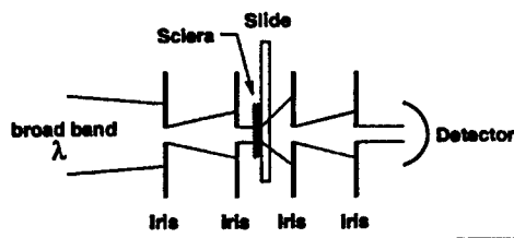
Figure 1: The tissue holder for the spectrophotometer only allows collimated light to strike the sclera and only collects the forward transmitted light. The incident beam is a converging incoherent broadband source.
