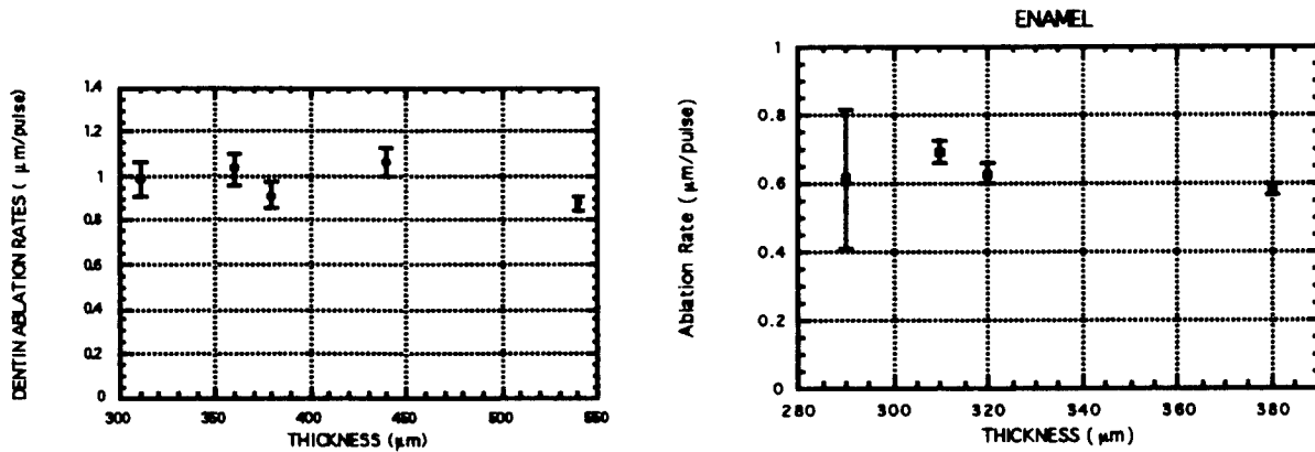
Figure 5 Dentin ablation rates as a function of ablated slice thickness
