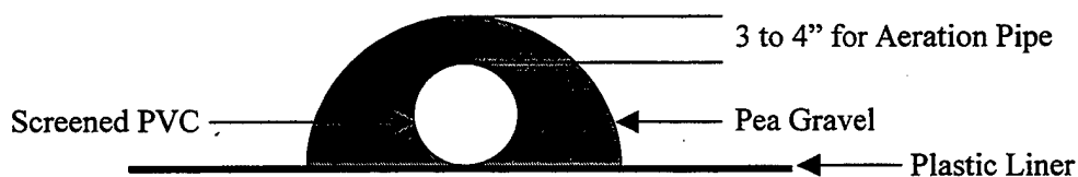
Figure 3-4. Placement of pea gravel.
