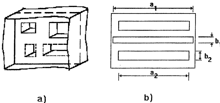
Fig. 1 Multiple rectangular aperture iris
