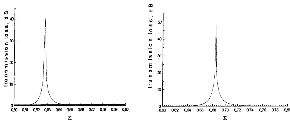
Fig. 4 Transmission loss for two different three aperture irises
