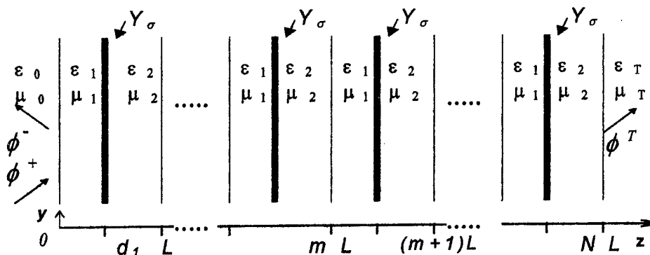
Fig.1 Multilayered structure.
