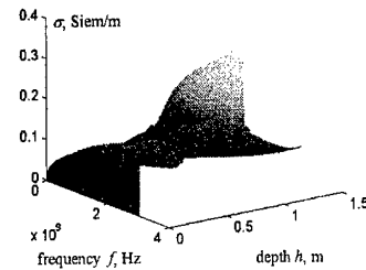
Fig. 7. Frequency-depth dependence of specific conductivity.
