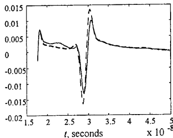
Fig. 5. The pulses reflected from the lower boundary of the layer of gray loam in the case of continuous humidity variation in depth according to Fig. 4 (solid line) and the fixed humidity W = 2.5\% (dotted line).
