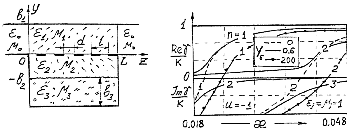
Fig. 1. Geometry. Dispersion dependences, b_1/l=20 ; b_2/l=b_3/l=3
