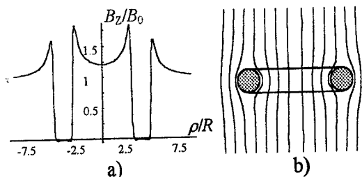
Fig. 2. Superconducting torus ( I=0 , B_0=1 ); (a) magnetic field profile in the central plane ( z=0 ); (b) magnetic field lines.
