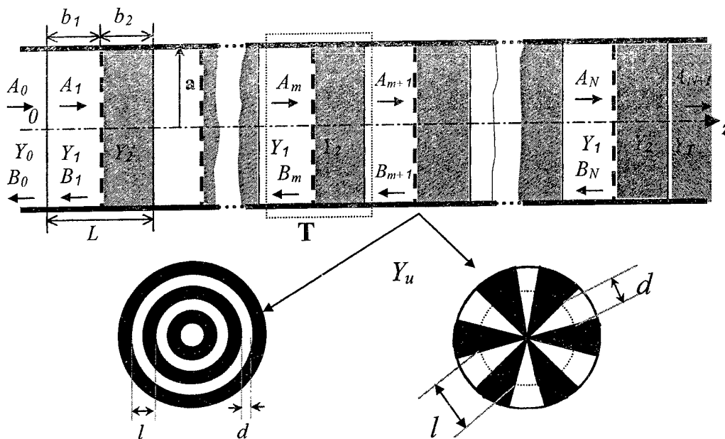
Fig. 1. Waveguide inhomogeneities
