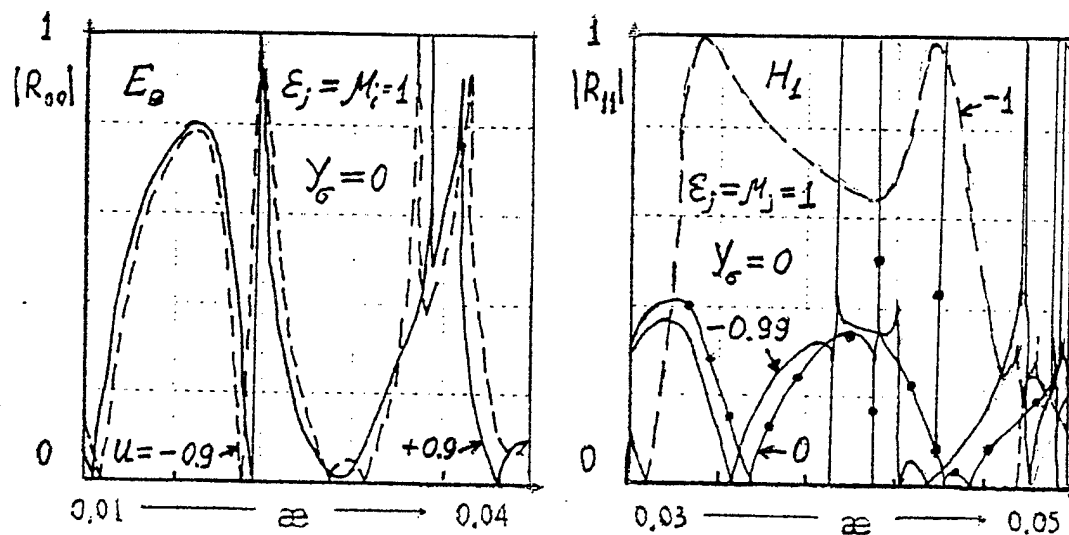
Fig. 2 Frequency dependences of |R| , b_1/l=20 ; b_2/l=b_3/l=5 ; L/l=4 .
