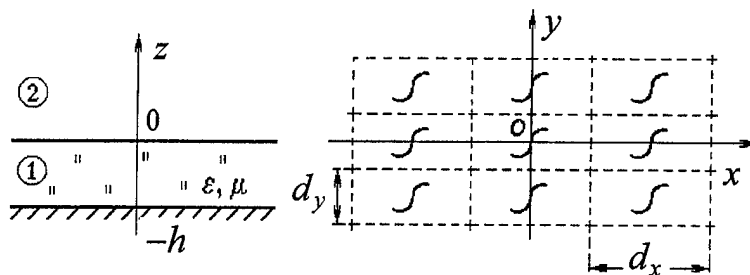
Fig. 1. Microstrip array.
