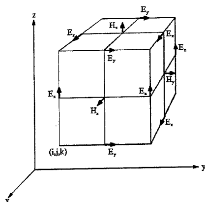
Fig.1. Node structures FDTD cell after Yee [5].
