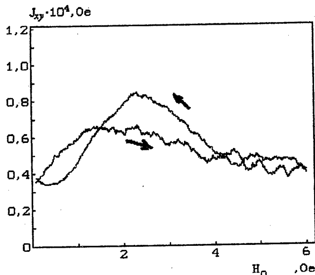
Fig.2. Dependence of the magnetization value J_{xy} on the intensity H_0 at the resonant frequency \omega = \gamma H_z .
