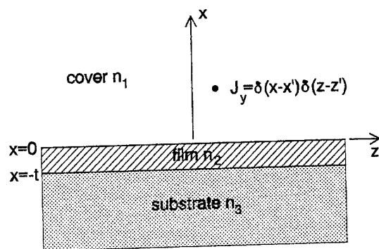
Fig. 1 Configuration of asymmetric planar dielectric waveguide with unit line-source excitation.
