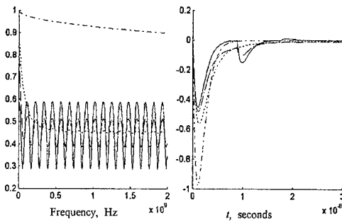
Fig.2. a) Frequency dependences of the absolute value of reflection factor |B_1(i\omega)| for a single-layer structure ( d_2 = 0.5 m, \varepsilon_1^r = 1 , \varepsilon_2^r = 7 , \varepsilon_3^r = 15 , \sigma_1 = 0 Siem/m) at various values of specific conductivities \sigma_2 and \sigma_3 : \sigma_2 = \sigma_3 = 0 Siem/m (continuous line), \sigma_2 = \sigma_3 = 1.2 \cdot 10^{-2} Siem/m (dotted line), \sigma_2 = \sigma_3 = 5 \cdot 10^{-2} Siem/m (dots), \sigma_2 = \sigma_3 = 20 Siem/m (dot-and-dash line); b) time dependence of diffraction fields.
