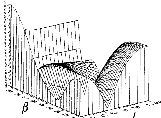
Fig. 6. Reflection coefficient of a two-layered curvilinear grating ( m_1=-m_2=0.25 ).
