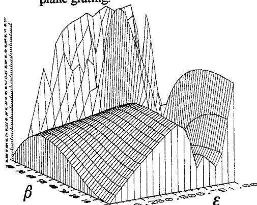
Fig. 5. Reflection coefficient of a two-layered curvilinear grating ( l=0.351d )
