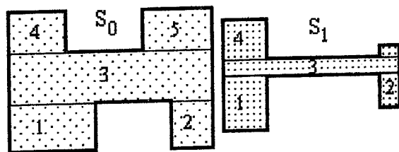
Fig.1. Cross-sections of two connected waveguides and their division into partial domains
