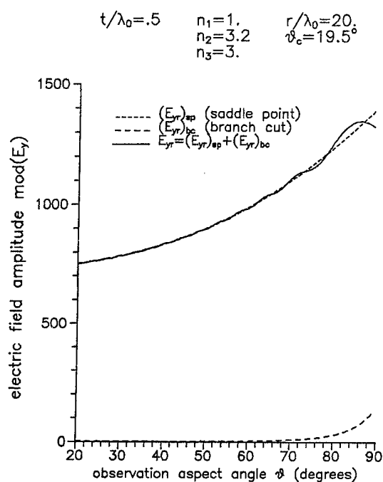
Fig. 8 Angular dependence of saddle-point and branch-cut contributions to the reflected wave component of the distant radiation field in the cover layer of an asymmetric planar dielectric waveguide.
