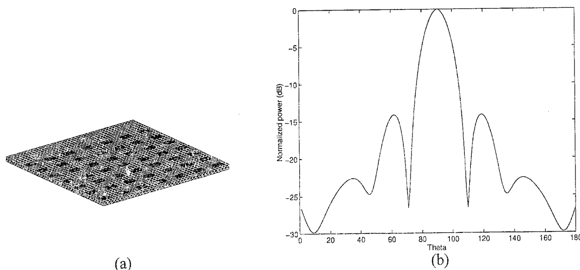
Figure 2: (a) 7 by 7 array of microstrip patches residing on a finite substrate and ground plane. A probe feed connects each patch to the ground plane, (b) Radiation pattern of the 7 by 7 array shown in (a).
