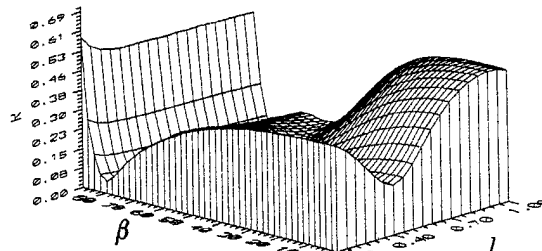
Fig. 4. Reflection coefficient of a two-layered curvilinear grating ( m_1=m_2=0.25 ).
