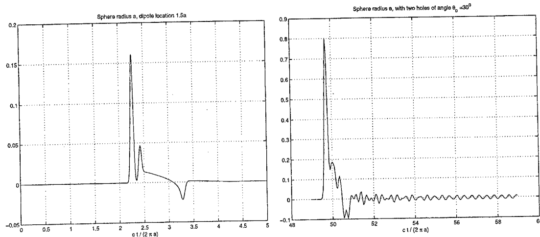
Figure 1: Radiated field at 10^\circ off-axis for the closed sphere (a) and the spherical cavity (b).
