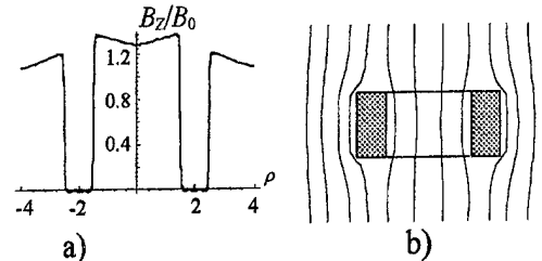
Fig. 5. Superconducting hollow cylinder ( B_0=1 , I=0 ); a) magnetic field profile in the central plane ( z=0 ); b) magnetic field lines.
