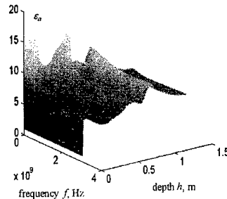
Fig. 6. Frequency-depth dependence of permittivity.
