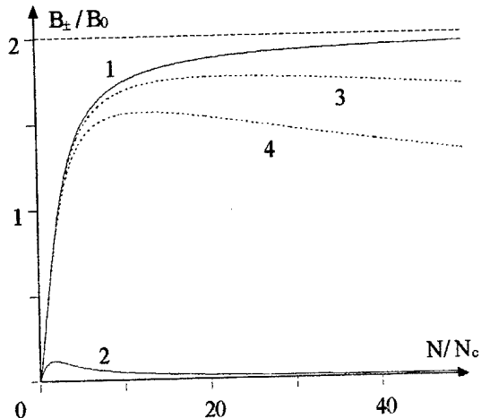
Fig. 2. The amplitude coefficient B_{+}/B_0 (curve 1) and B_{-}/B_0 (curve 2) vs parameter N/N_c for original plane wave. The dashed curves show the coefficient B_{+}/B_0 for the original wave beam with h_0 a = 10 (curve 3) and h_0 a = 5 (curve 4).
