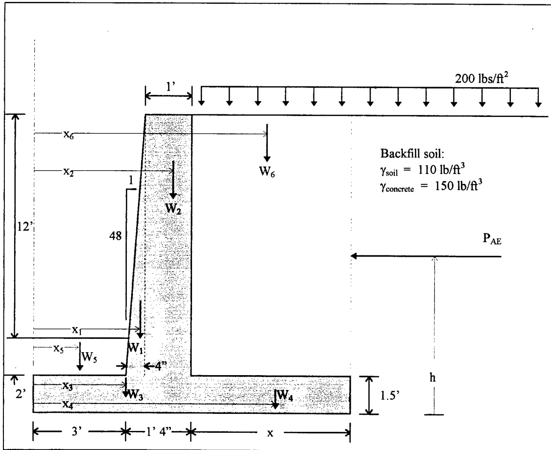
Figure 3-3: Concrete cantilever retaining wall.
