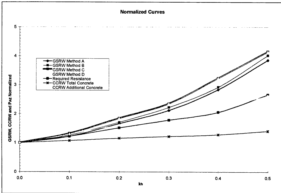
Figure 3-10: Normalized curves.
