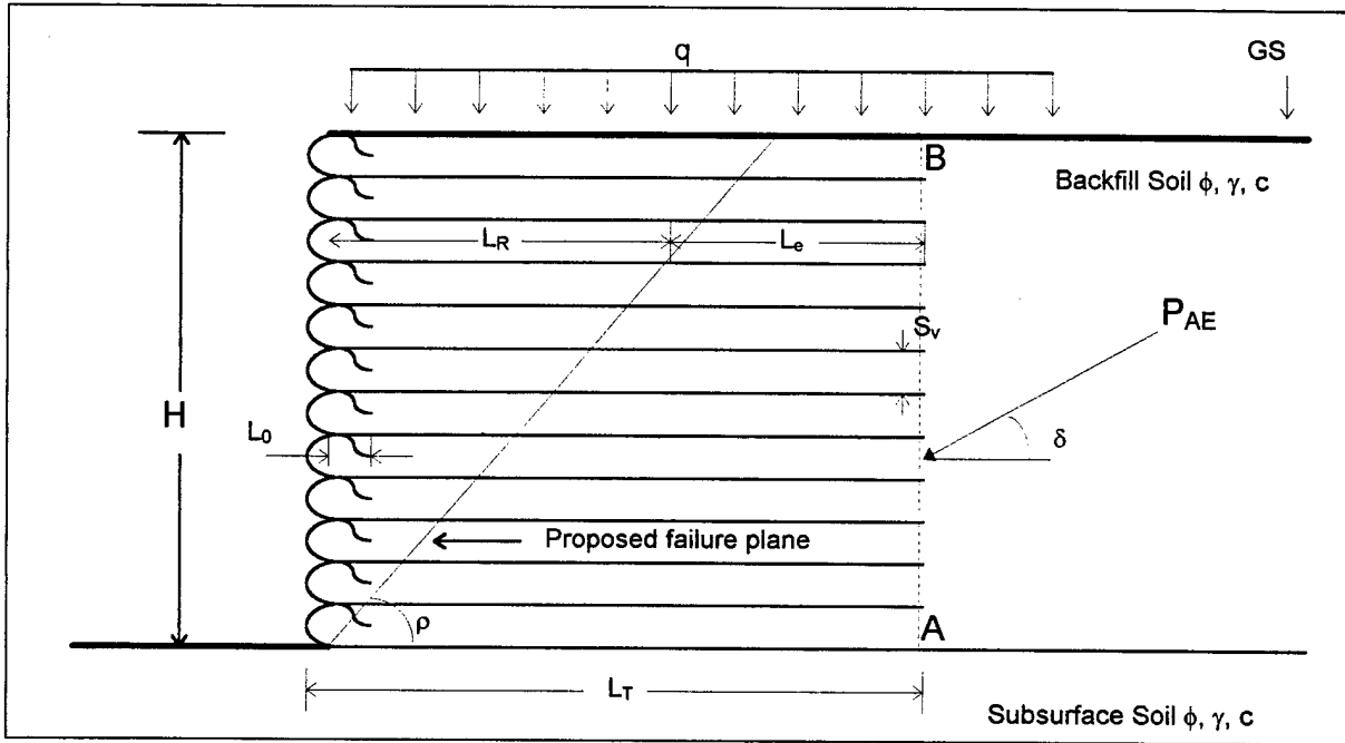
Figure 2-7: Typical geosynthetic reinforced retaining structure.
