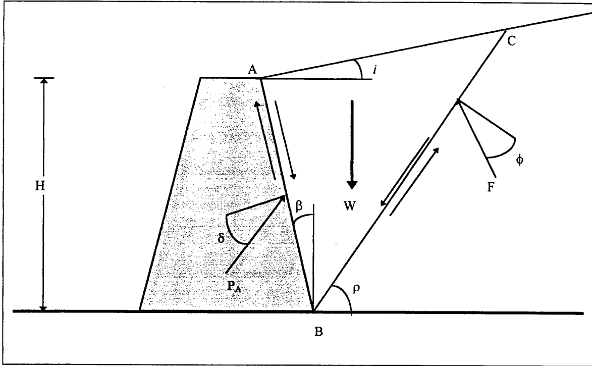
Figure 2-3: Coulomb's active earth pressure.
