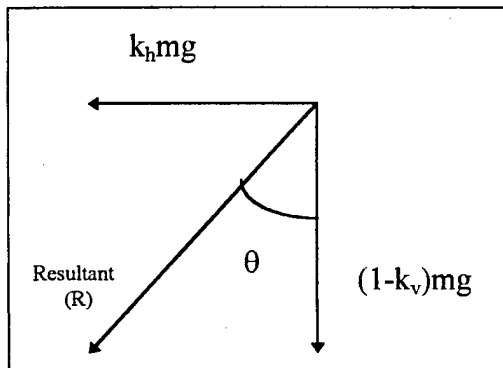
Fig 2-5a Coulomb
