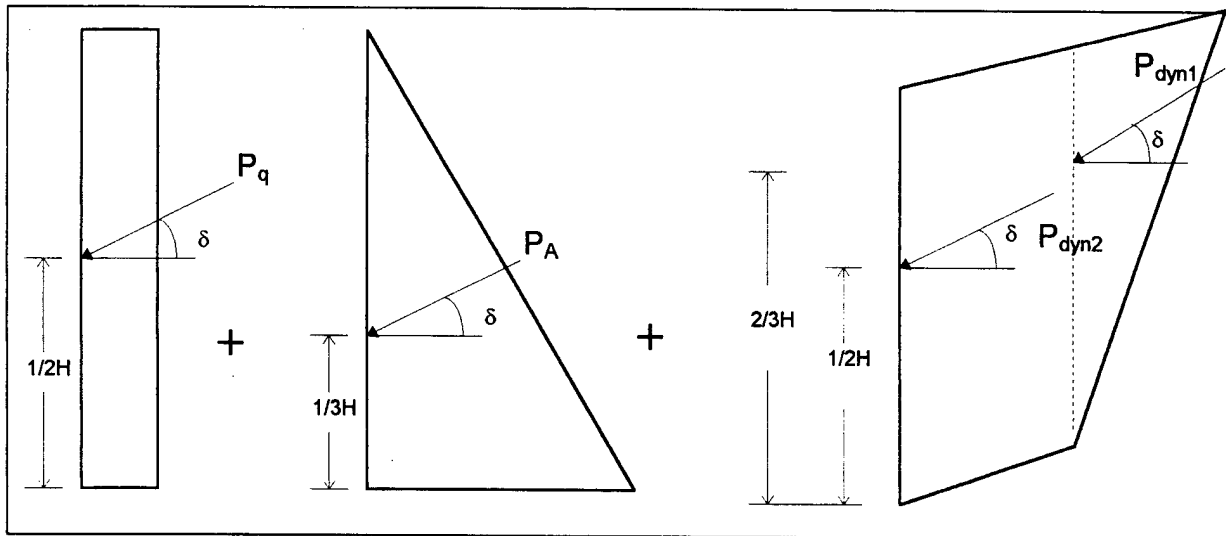
Figure 2-8: Static and dynamic pressure distribution.
