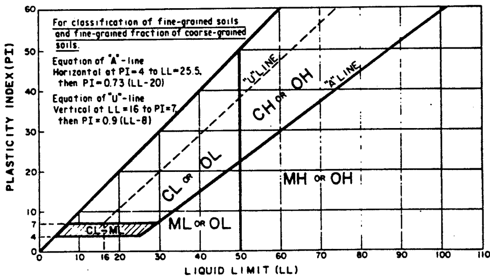
FIG. 6—Plasticity chart.
