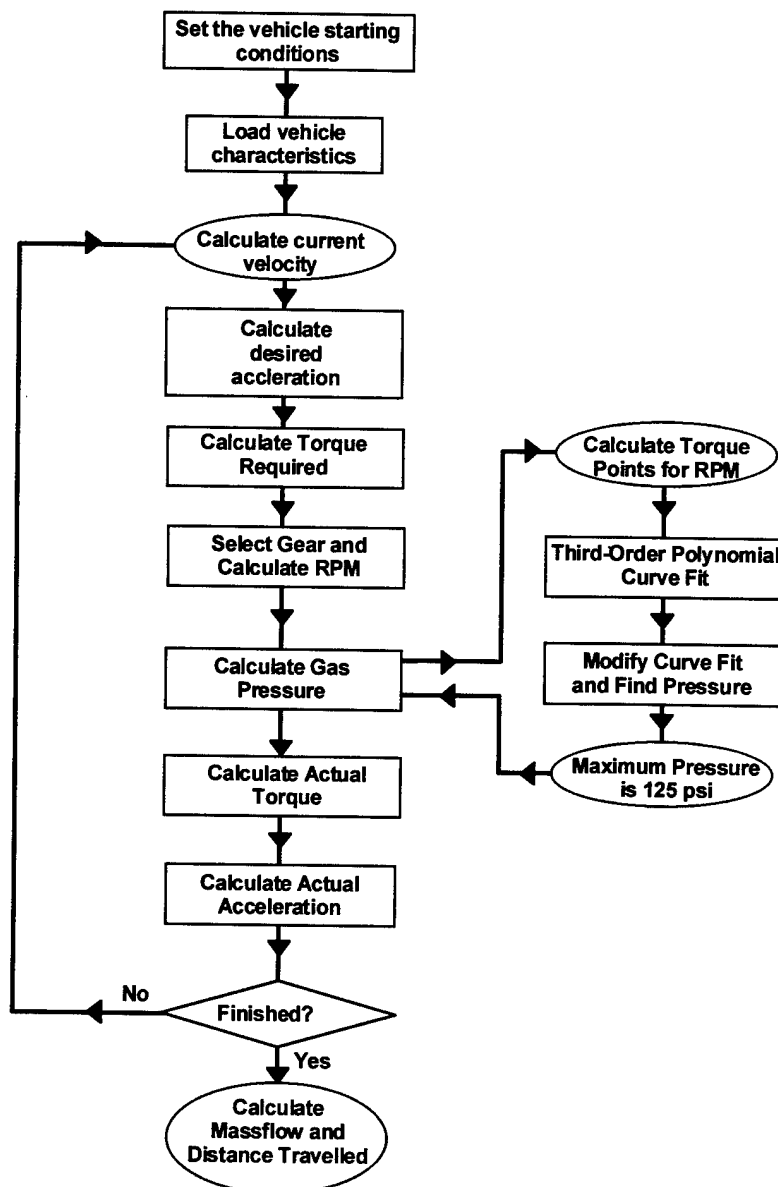
Figure 12: Performance Prediction Algorithm.
