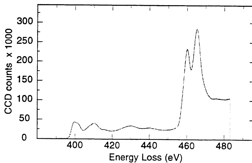
Figure 4.85 PEELS analysis of inclusion JWV2 Region B - \text{N}_\text{K} spectrum
