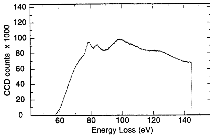
Figure 4.69 PEELS analysis of inclusion JWV1 Region A - \text{Al}_{\text{L}_{2,3}} spectrum
