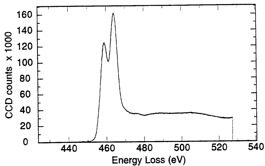
Figure 4.54 PEELS analysis of inclusion JWZ2 Region B - \text{Ti}_{L2,3} spectrum
