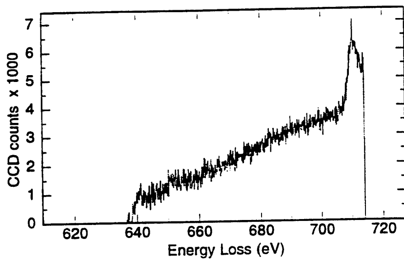
Figure 4.28 PEELS analysis of inclusion JWY2 - \text{Mn}_{\text{L2,3}} spectrum
