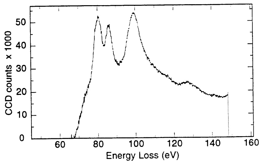
Figure 4.57 PEELS analysis of inclusion JWZ2 Region B - \text{Al}_{L2,3}
