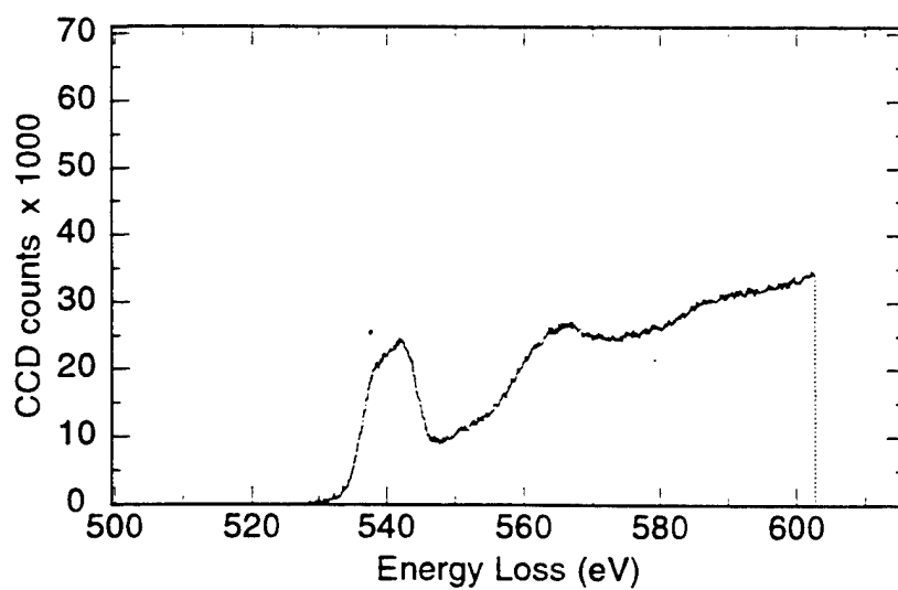
Figure 4.95 PEELS analysis of inclusion J WV3 Region A - O K spectrum
