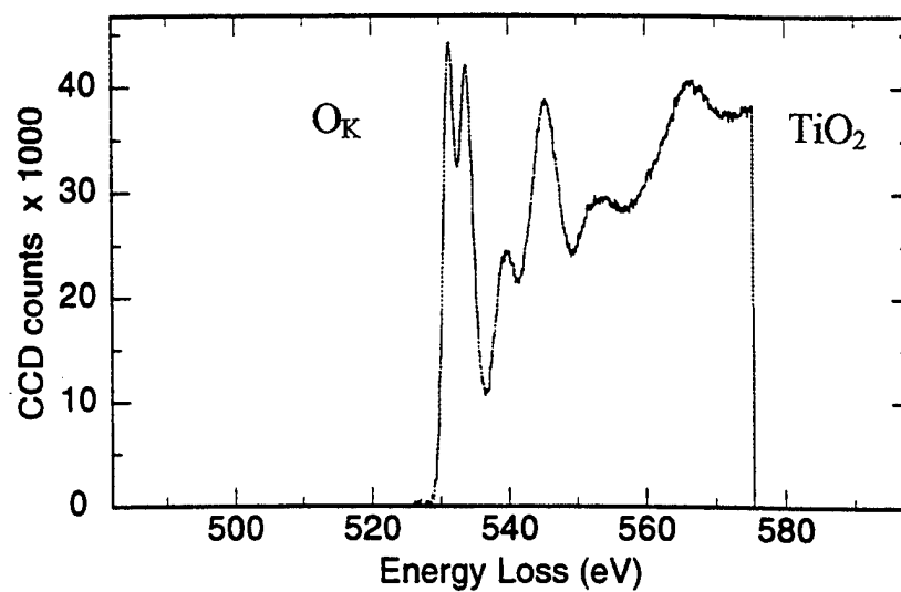
Figure 4.15 Energy loss spectra for oxygen - \text{TiO}_2
