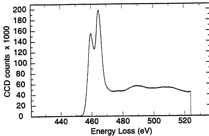
Figure 4.43 PEELS analysis of inclusion JWZ1 - \text{Ti}_{L2,3} spectrum
