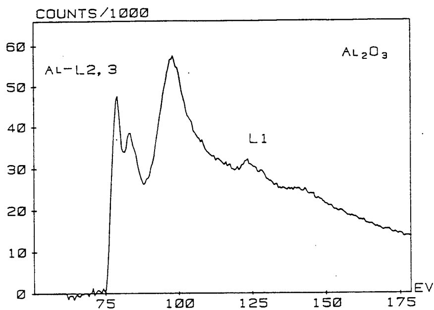
Figure 4.16 Energy loss spectra for aluminum - \text{Al}_2\text{O}_3 [From Ref. 38]
