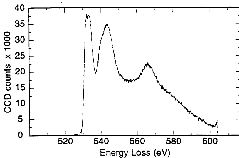
Figure 4.32 PEELS analysis of inclusion JWY3 Region A - \text{O}_\text{K} spectrum
