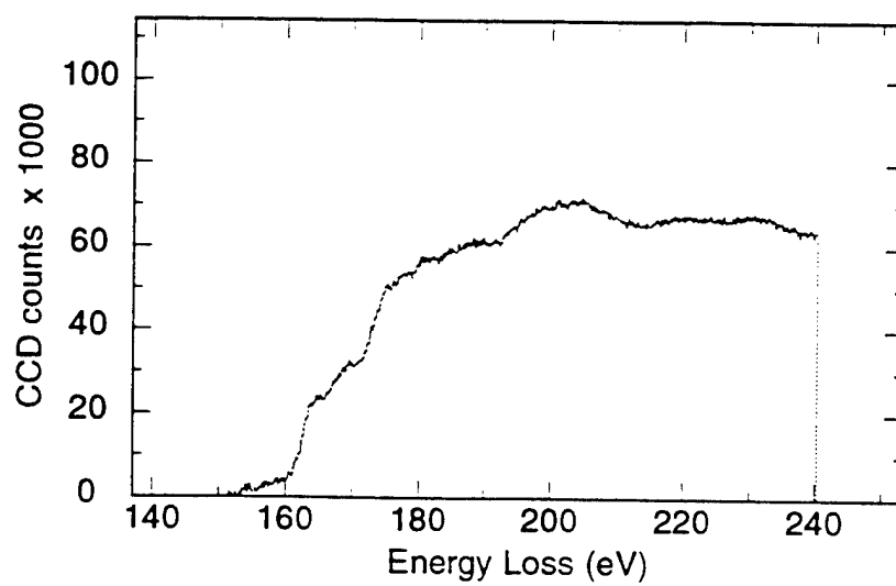
Figure 4.91 PEELS analysis of inclusion J WV2 Region C - S L spectrum
