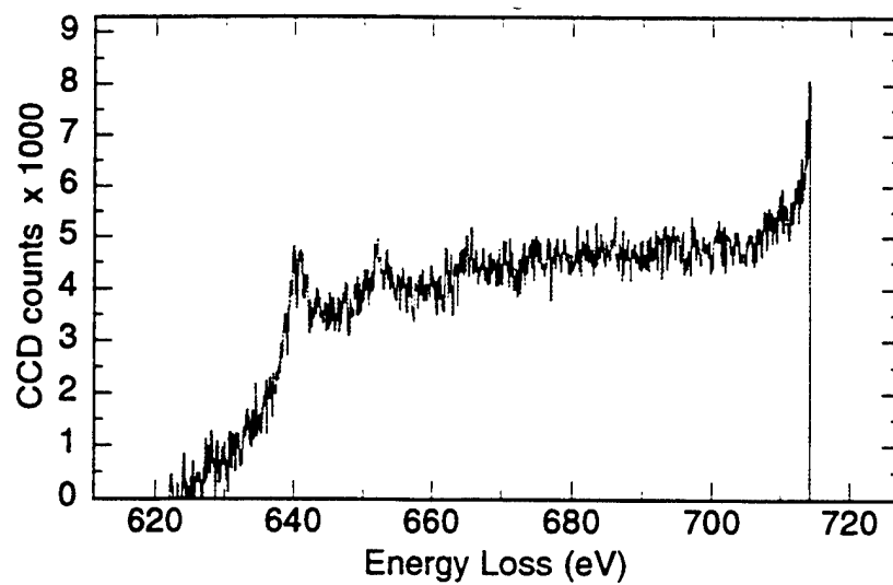
Figure 4.45 PEELS analysis of inclusion JWZ1 - \text{Mn}_{\text{L}_{2,3}} spectrum
