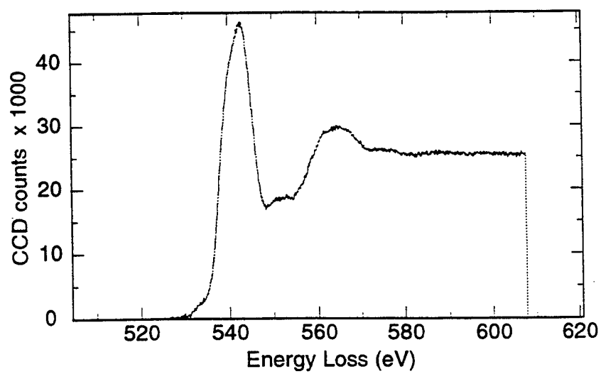
Figure 4.83 PEELS analysis of inclusion J WV2 Region B - O_K spectrum
