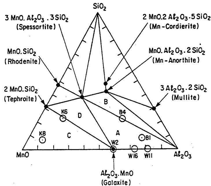
Figure 2.11 Ternary Diagram of Coexisting Phases in Annealed Mixes for the System \text{Al}_2\text{O}_3\text{-MnO-SiO}_2 [From Ref. 29]
