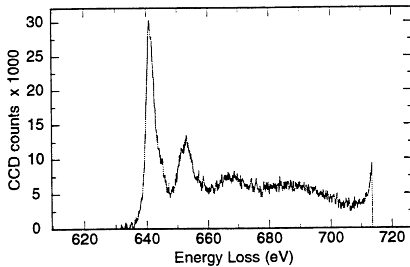
Figure 4.37 PEELS analysis of inclusion JWY3 Region B - \text{Mn}_{\text{L}_{2,3}} spectrum
