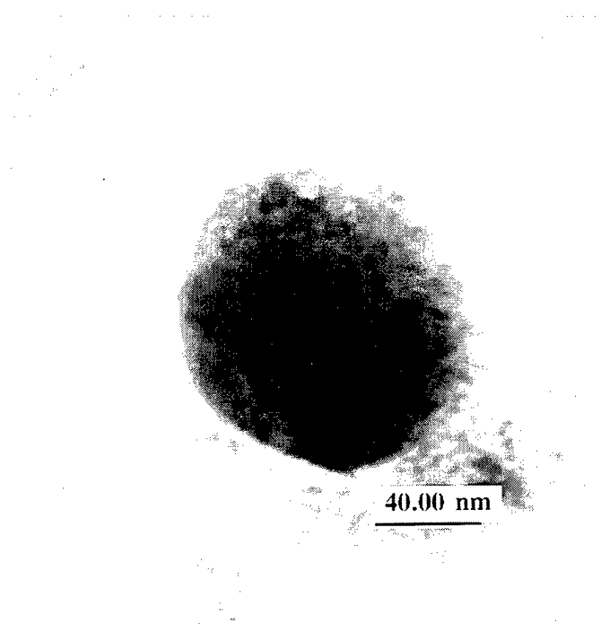
Figure 4.58 TEM microrgraph of inclusion JWZ3
