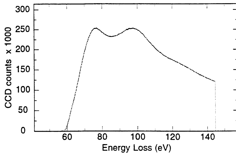
Figure 4.73 PEELS analysis of inclusion J WV1 Region B - \text{Al}_{\text{L}_{2,3}} spectrum
