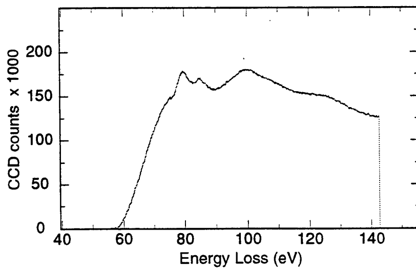
Figure 4.96 PEELS analysis of inclusion J WV3 Region A - \text{Al}_{\text{L}_{2,3}} spectrum
