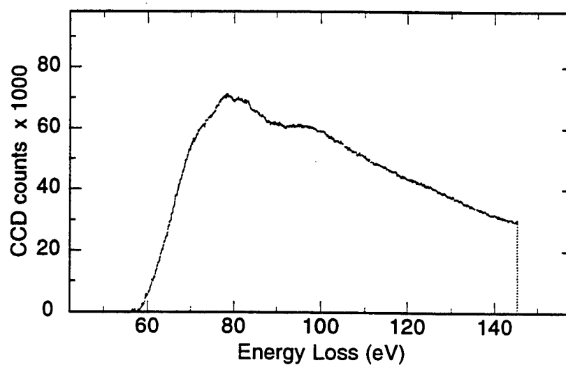
Figure 4.90 PEELS analysis of inclusion J WV2 Region C - \text{Al}_{\text{L}_{2,3}} spectrum
