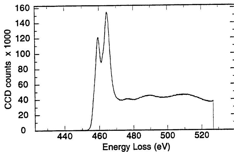
Figure 4.21 PEELS analysis of inclusion JWY1 - \text{Ti}_{\text{L}_{2,3}} spectrum
