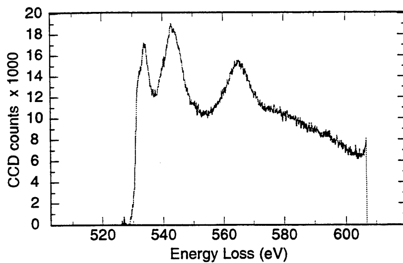
Figure 4.22 PEELS analysis of inclusion JWY1 - \text{O}_{\text{K}} spectrum
