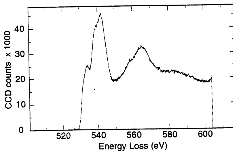
Figure 4.44 PEELS analysis of inclusion JWZ1 - \text{O}_K spectrum
