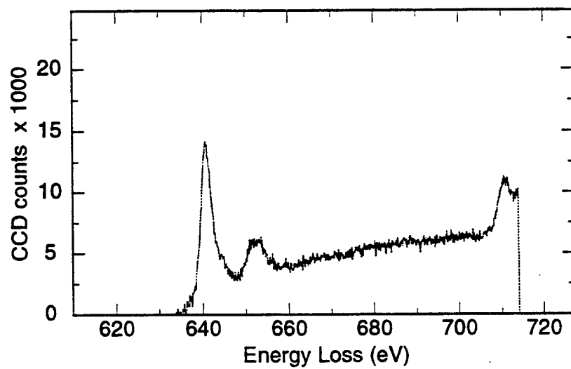
Figure 4.33 PEELS analysis of inclusion JWY3 Region A - \text{Mn}_{\text{L2,3}} spectrum
