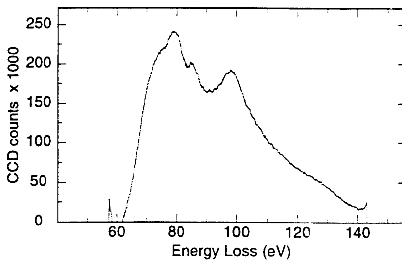
Figure 4.46 PEELS analysis of inclusion JWZ1 - \text{Al}_{\text{L}_{2,3}} spectrum
