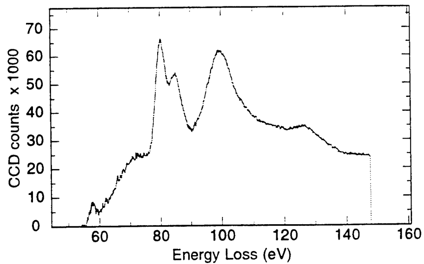
Figure 4.84 PEELS analysis of inclusion JWV2 Region B - \text{Al}_{\text{L2,3}} spectrum
