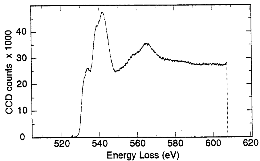
Figure 4.55 PEELS analysis of inclusion JWZ2 Region B - \text{O}_K spectrum
