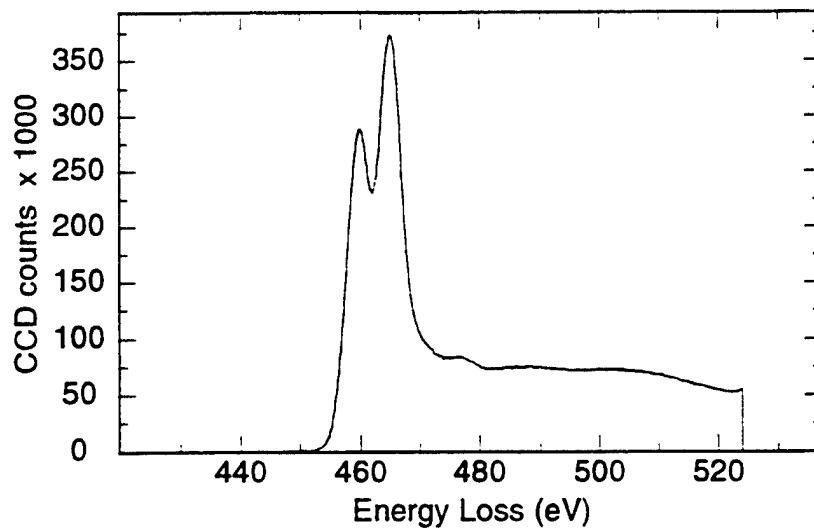
Figure 4.31 PEELS analysis of inclusion JWY3 Region A - \text{Ti}_{\text{L2,3}} spectrum
