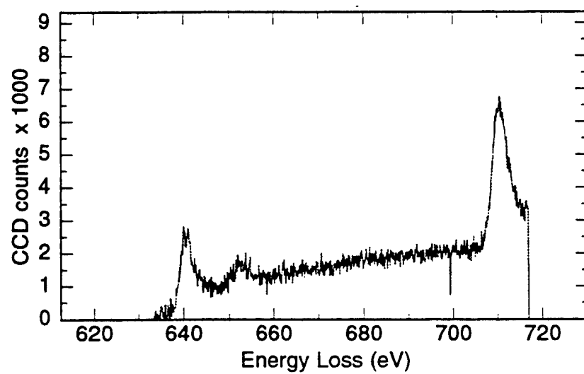
Figure 4.23 PEELS analysis of inclusion JWY1 - \text{Mn}_{\text{L}_{2,3}} spectrum
