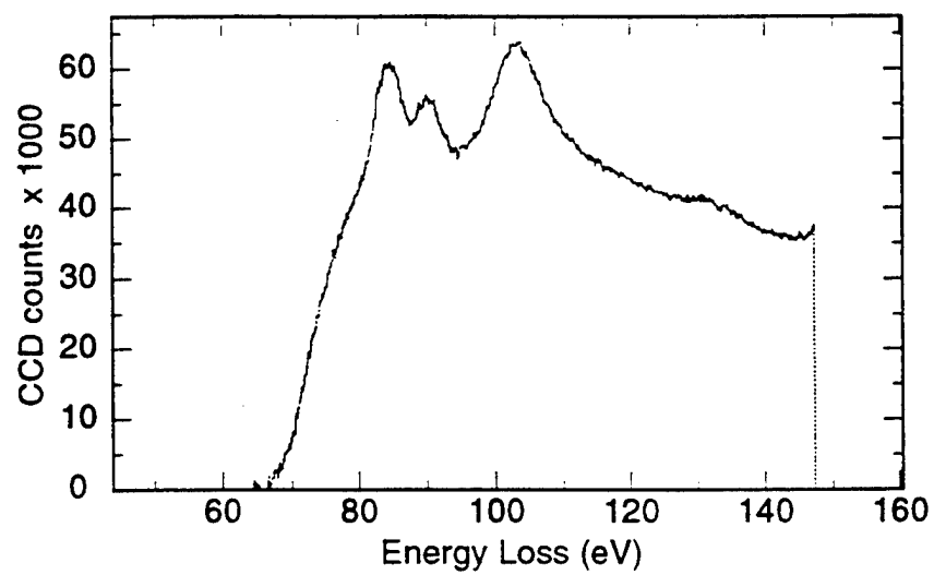
Figure 4.62 PEELS analysis of inclusion JWZ3 - \text{Al}_{\text{L}_{2,3}} spectrum
