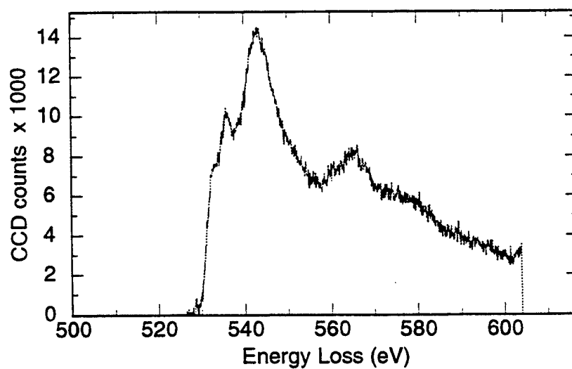
Figure 4.36 PEELS analysis of inclusion JWY3 Region B - \text{O}_\text{K} spectrum
