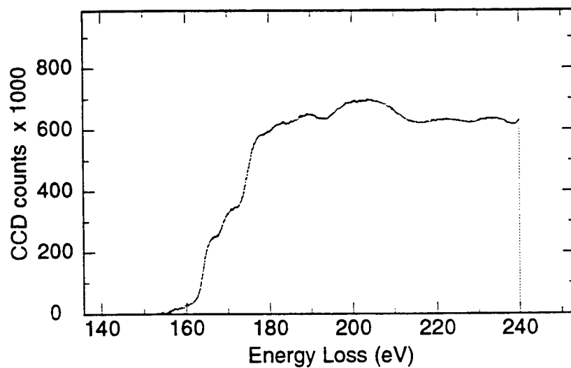
Figure 4.38 PEELS analysis of inclusion JWY3 Region B - \text{S}_{\text{L}_{2,3}} spectrum
