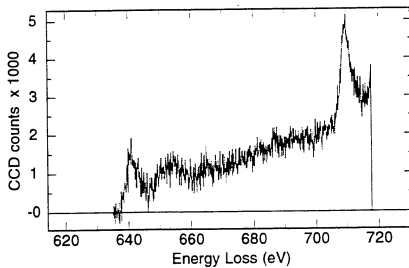
Figure 4.56 PEELS analysis of inclusion JWZ2 Region B - \text{Mn}_{L2,3} spectrum
