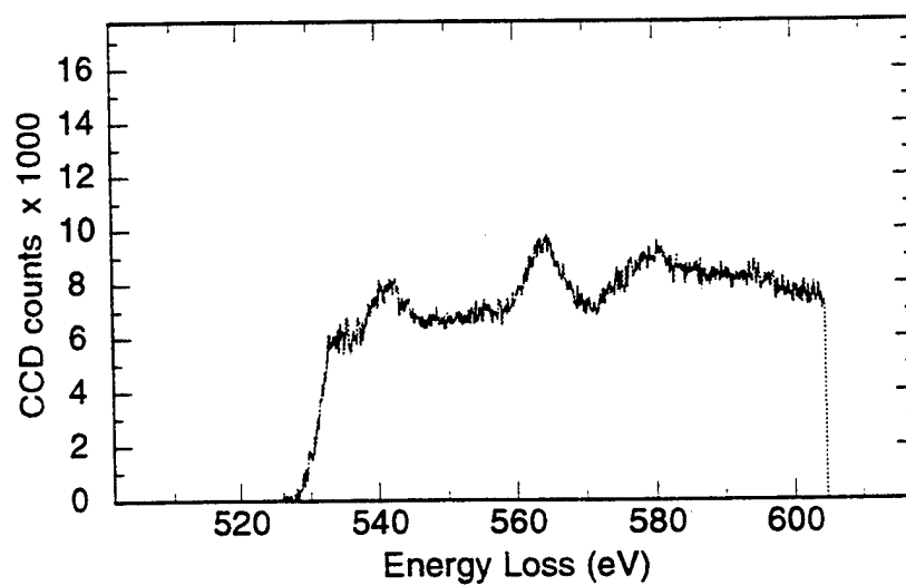
Figure 4.72 PEELS analysis of inclusion J WV1 Region B - \text{O}_K spectrum
