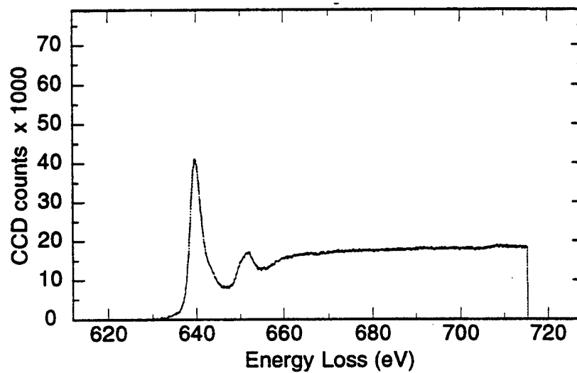
Figure 4.89 PEELS analysis of inclusion J WV2 Region C - \text{Mn}_{\text{L}_{2,3}} spectrum
