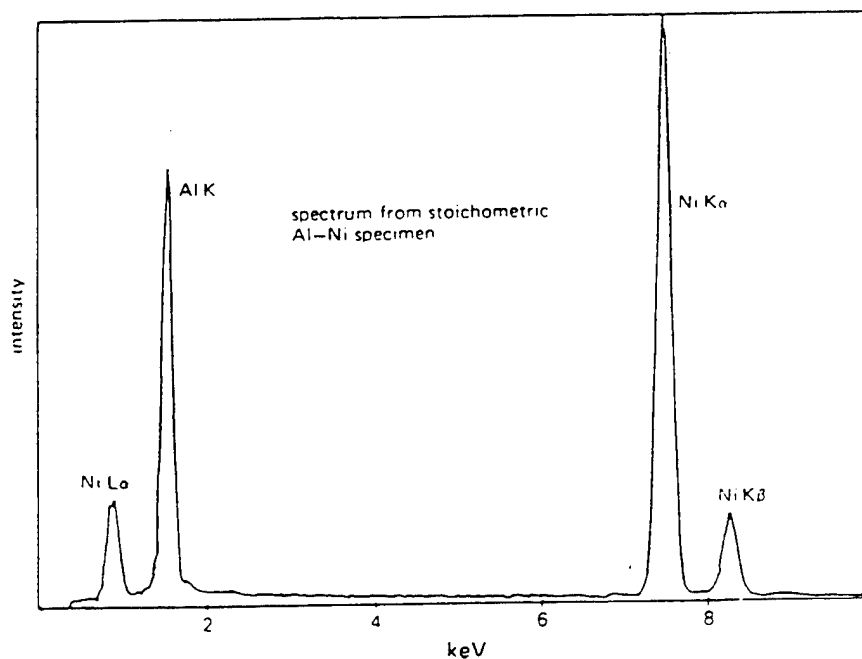
Figure 3.9 Typical EDX spectrum [From Ref. 37]
