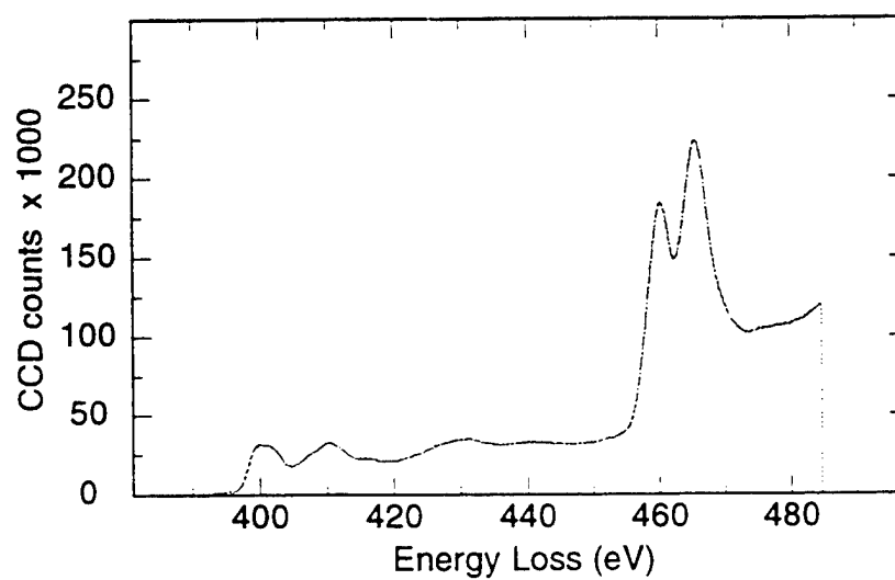
Figure 4.74 PEELS analysis of inclusion J WV1 Region B - \text{N}_{\text{K}} spectrum
