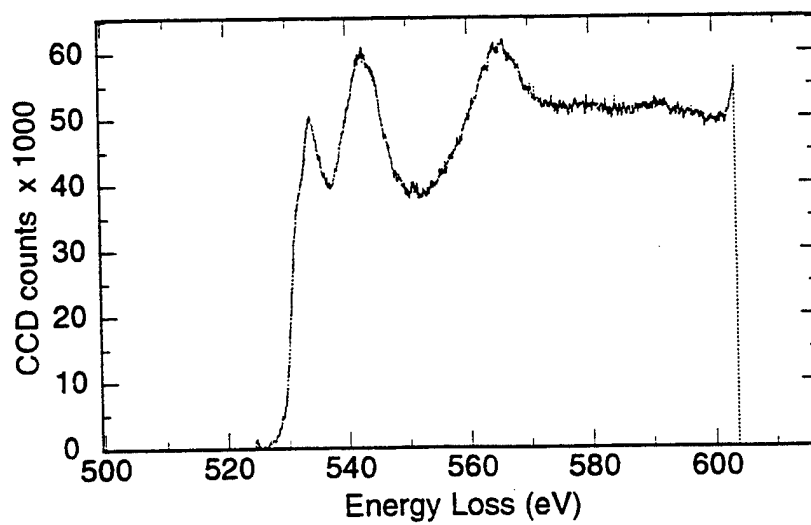
Figure 4.27 PEELS analysis of inclusion JWY2 - \text{O}_{\text{K}} spectrum
