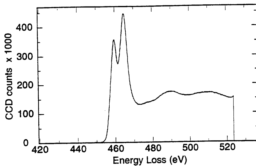
Figure 4.26 PEELS analysis of inclusion JWY2 - \text{Ti}_{\text{L}_{2,3}} spectrum
