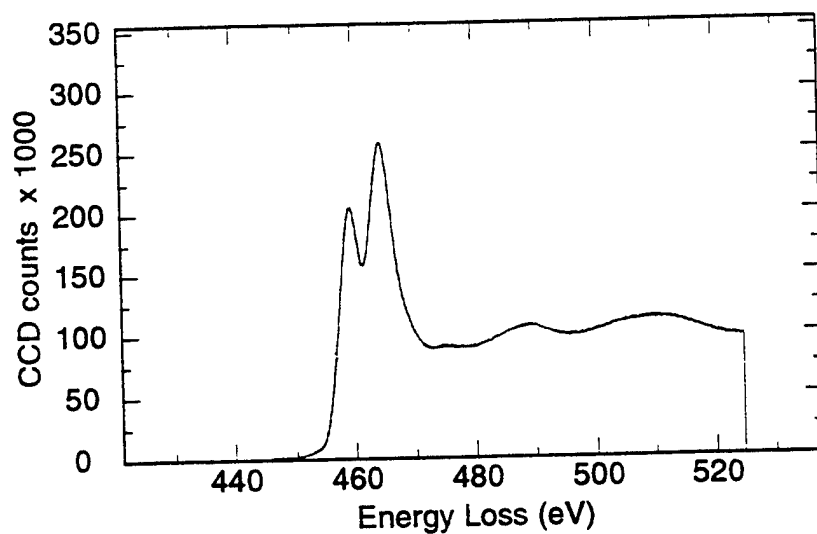
Figure 4.71 PEELS analysis of inclusion J WV1 Region B- \text{Ti}_{\text{L2,3}} spectrum
