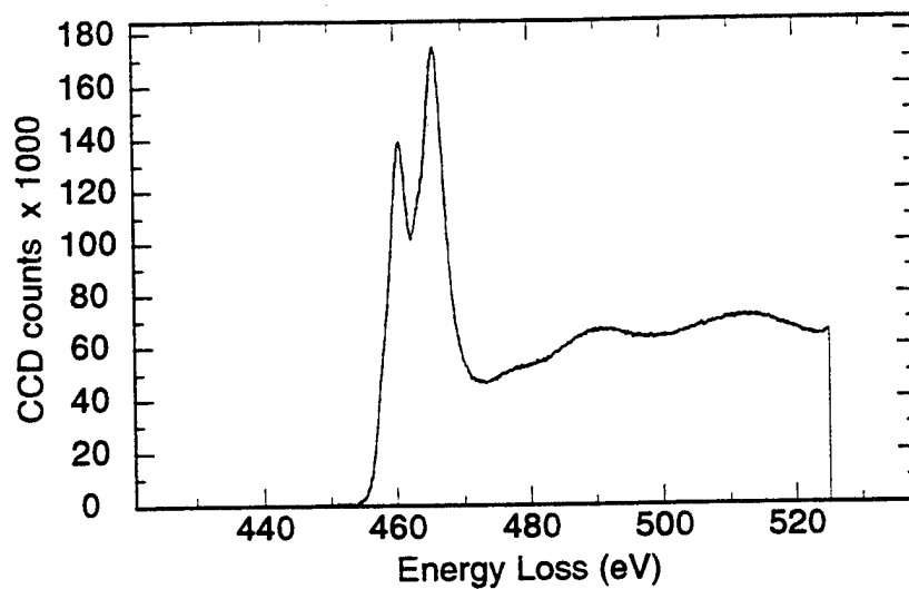
Figure 4.35 PEELS analysis of inclusion JWY3 Region B- \text{Ti}_{\text{L}_{2,3}} spectrum
