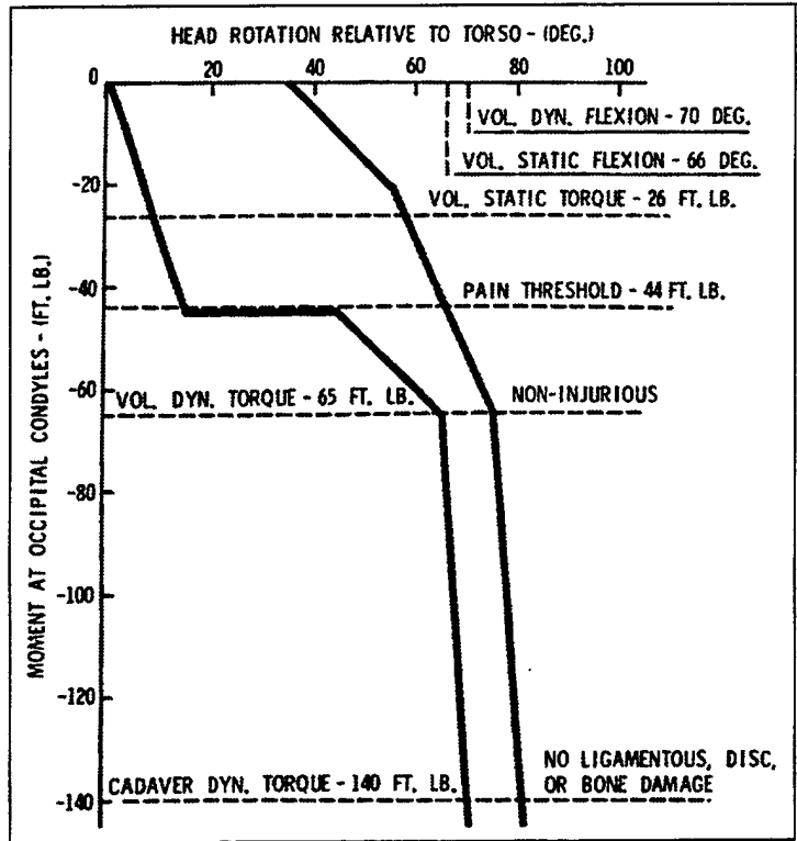
Figure 40. Flexion Response Envelope. From Ref. [16]
