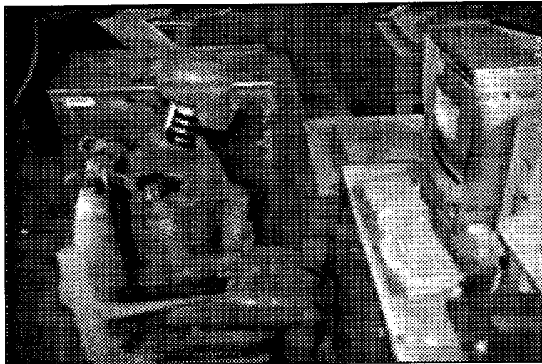
Figure 6. Seated Hybrid III Dummy Setup
