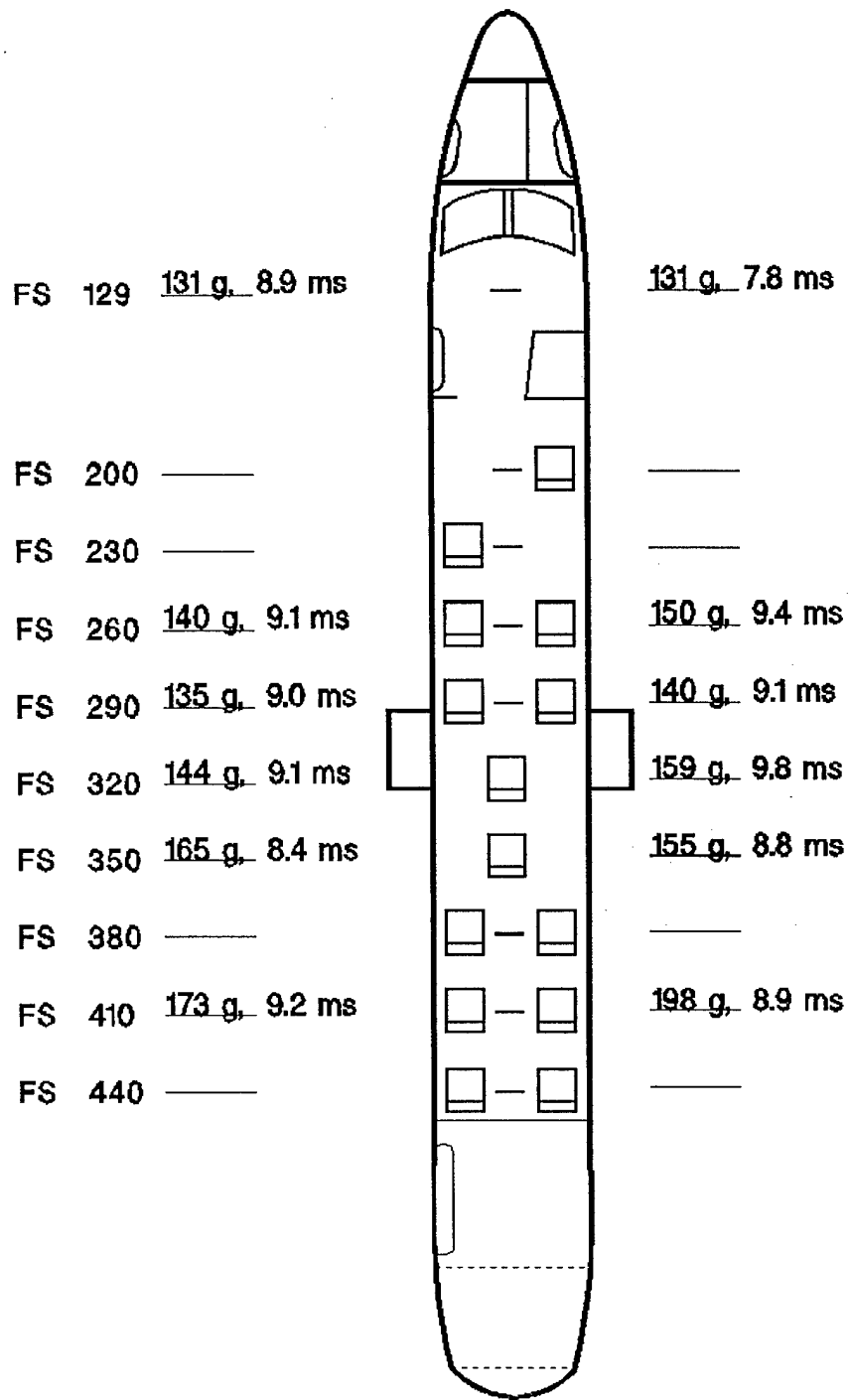
FIGURE 6. FLOOR SEAT TRACK ACCELERATIONS ( G_{max} )
