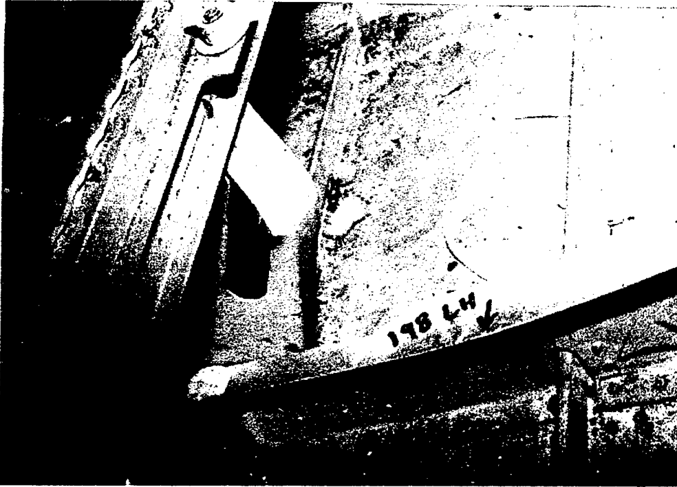
FIGURE 20. UNDERFLOOR BUCKLING L/H SIDE, AFTER IMPACT
