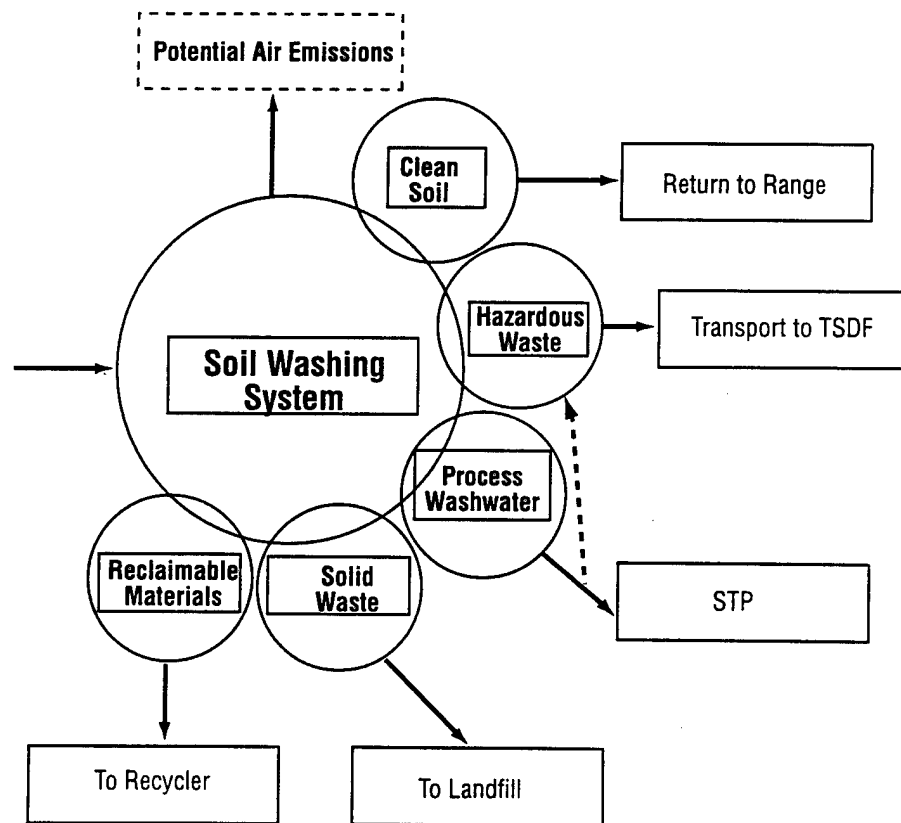
Figure 3. Soil Washing Process Flow Diagram
