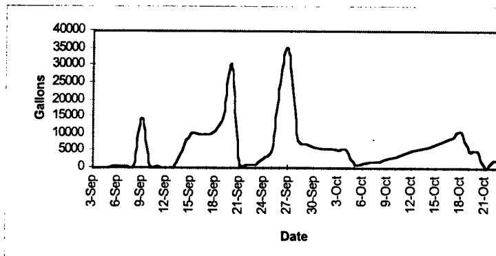
Figure 5. Estimated Runoff Pond Volume Acetic Acid Demonstration
