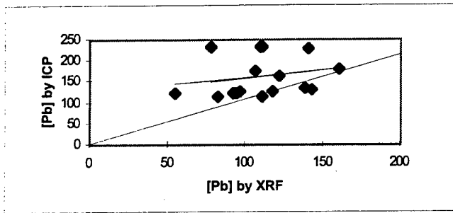
Figure 26. Battelle ICP vs. Battelle X-RF; Y=0.35X+122.23, R^2=0.04
