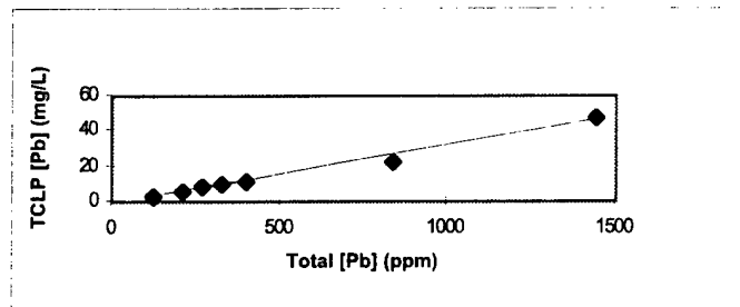
Figure 29. TCLP vs. Total (Pb) Acetic Acid Demonstration; Y=0.03X-1.48, R^2=0.98
