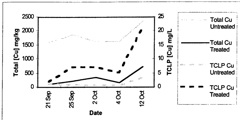
Figure 40. Levels of Copper in Range Soil (Acetic Acid Leaching)
