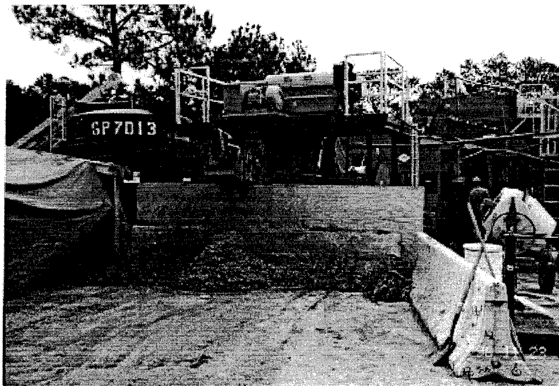
Figure 39. Centrifuge
