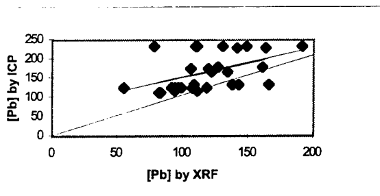
Figure 28. ICP vs. X-RF (All Data); Y=0.75X+75.54, R^2=0.23
