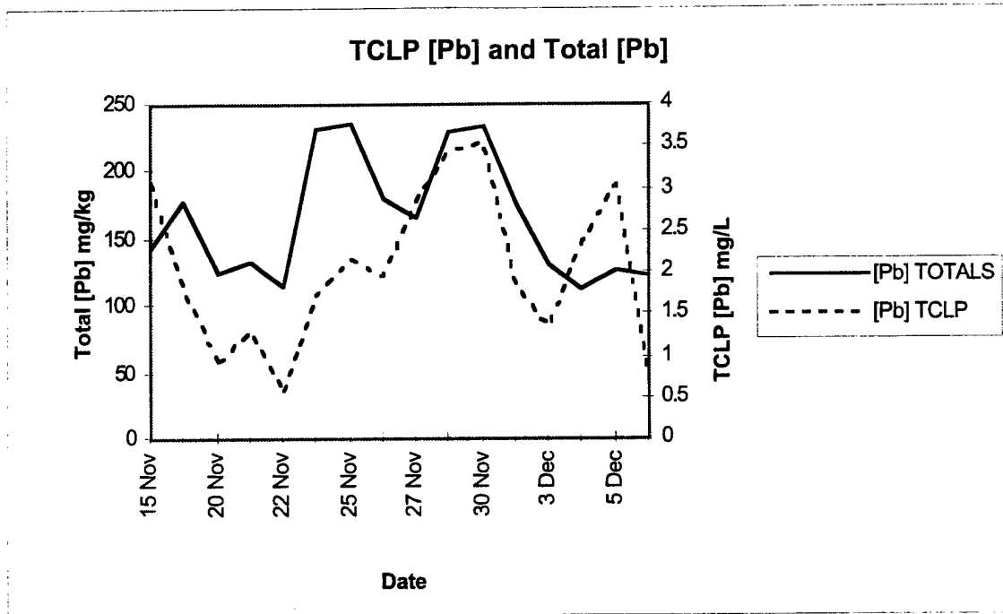
Figure 47. Total Lead and TCLP Lead Treatment Results (Hydrochloric Acid Demonstration)
