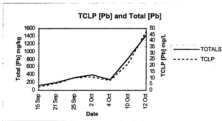
Figure 46. Total Lead and TCLP Lead Treatment Results (Acetic Acid Demonstration)
