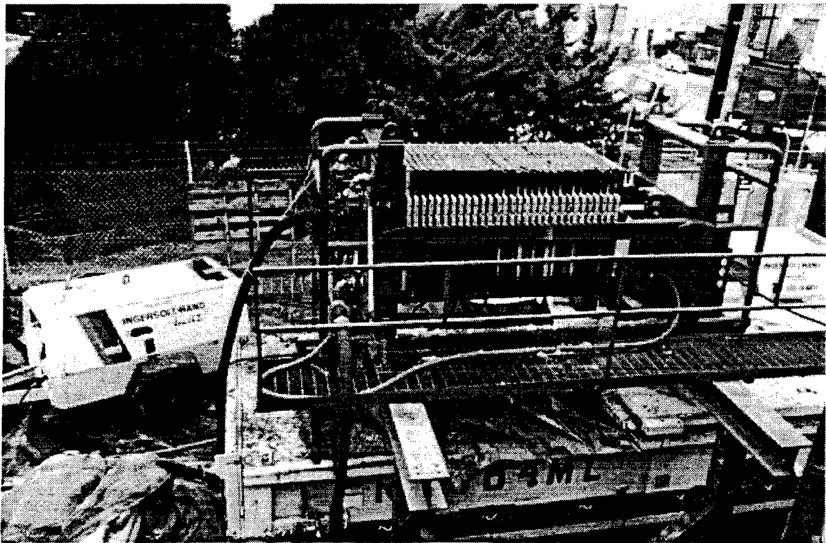
Figure 35. Frame Filter Press
