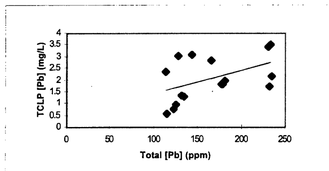
Figure 30. TCLP vs. Total (Pb) Hydrochloric Acid Demonstration; Y=0.40X+0.01, R^2=0.24
