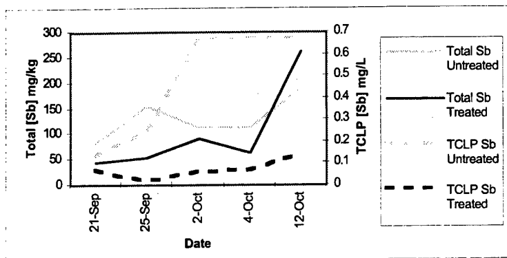
Figure 41. Levels of Antimony in Range Soil (Acetic Acid Leaching)
