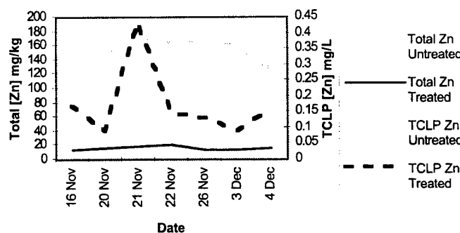
Figure 45. Levels of Zinc in Range Soil (Hydrochloric Acid Leaching)
