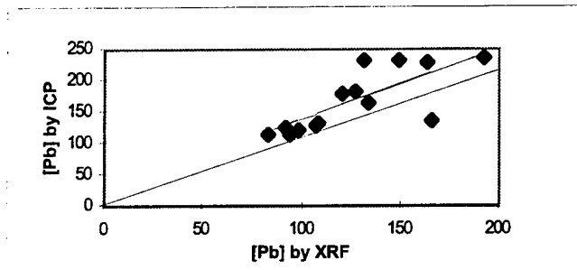
Figure 27. Battelle ICP vs. BESCORP X-RF; Y=1.13X+22.89, R^2=0.57
