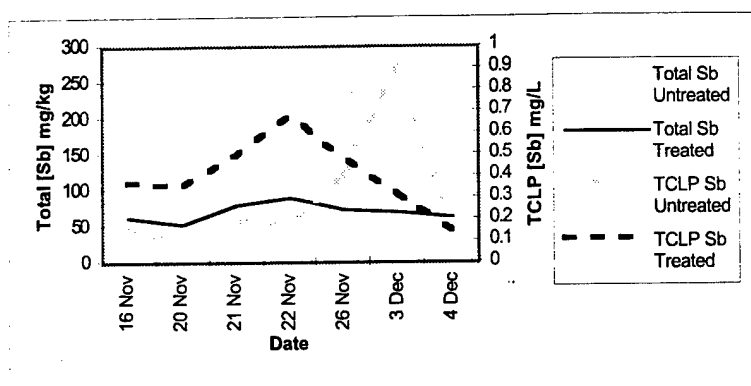
Figure 44. Levels of Antimony in Range Soil (Hydrochloric Acid Leaching)
