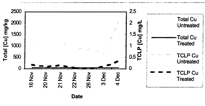
Figure 43. Levels of Copper in Range Soil (Hydrochloric Acid Leaching)
