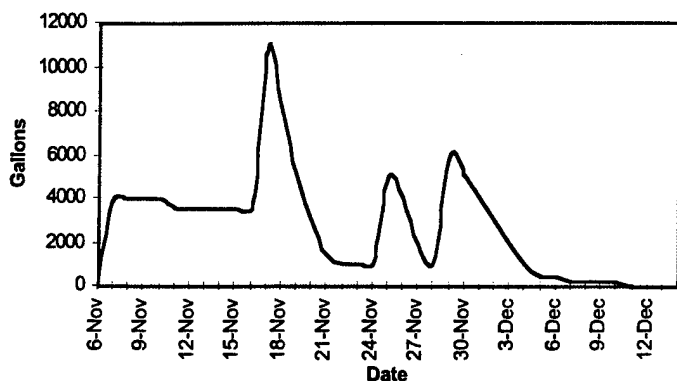
Figure 6. Estimated Runoff Pond Volume Hydrochloric Acid Demonstration
