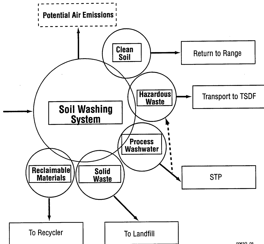
Figure 3. Soil Washing Process Flow Diagram
