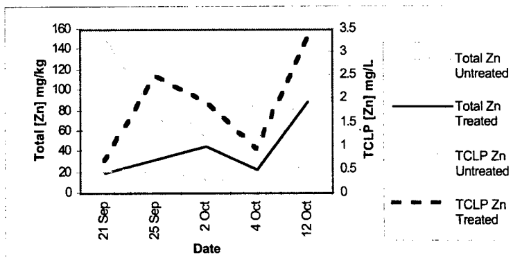
Figure 42. Levels of Zinc in Range Soil (Acetic Acid Leaching)
