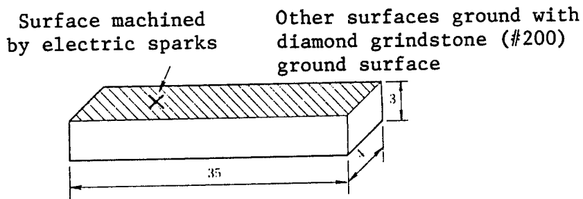
(a) Bending Test Specimen Surface Machined by Electric Sparks
