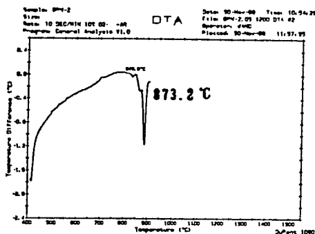
Fig.3. DTA pattern of the sample by NCD under 10% O2+Ar atmosphere
