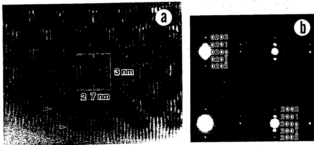
Fig.1 (a) A lattice image of \text{Bi}_2(\text{Sr,Ca})_3\text{Cu}_2\text{O}_x , taken by the incident beam parallel to the \underline{a} axis. (b) A diffraction pattern, taken with the incident beam parallel to the \underline{c} direction.
