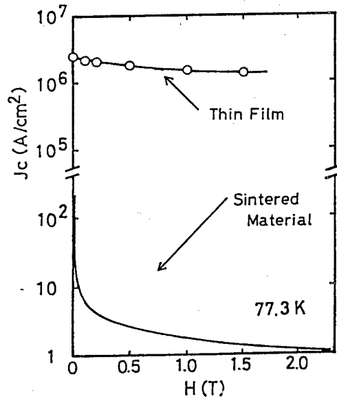
Fig.7 Magnetic field dependence of J_c for HoBaCuO thin film
