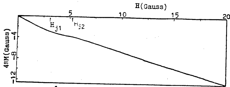
Fig. 1 Magnetization curve of YBaCuO at low field.
