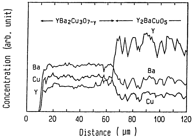
Fig. 2 Concentration profile of YBCO diffusion layer formed on a Y_2BaCuO_5 substrate. The specimen was heat treated at 930^\circ\text{C} for 6hrs.
