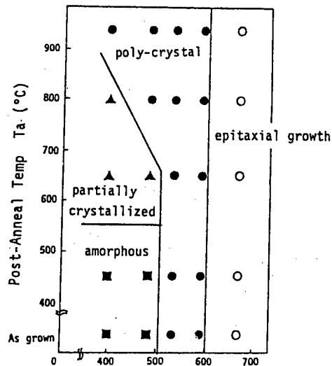
Fig.1 Substrate temperature and post-anneal temperature dependence of film crystallinity
