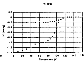
Fig. 4 Magnetization versus temperature of the TlBa_2Ca_3Cu_4O_{11} (1234) sample under 100 Gauss.
