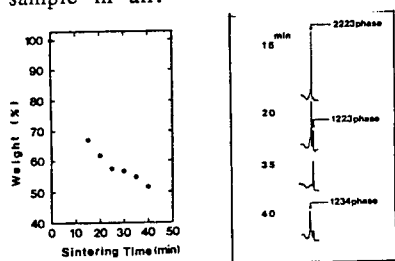
Fig. 1 Weight % ( W_{\text{sintered}}/W_{\text{initial}} ) of the sample pellet vs sintering time
