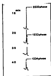
Fig. 2 Change of the x-ray diffraction patterns with sintering time.
