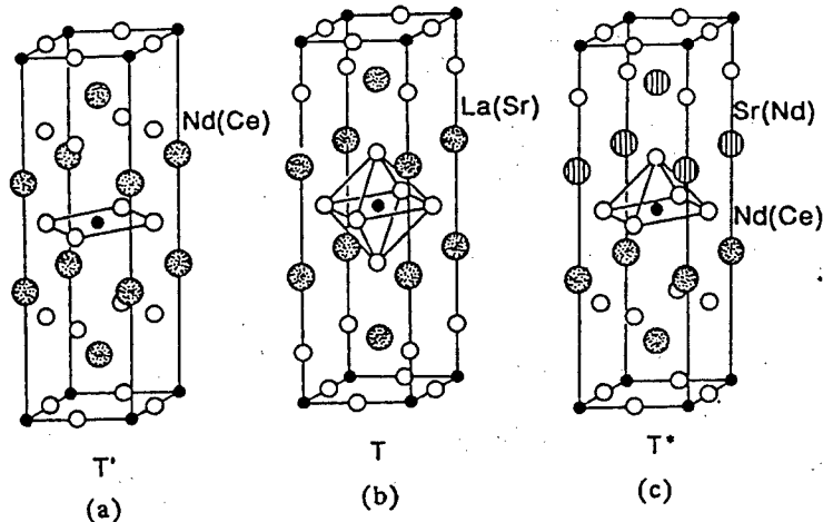
Fig.1: Crystal structures of (a) Nd_{2-x}Ce_xCuO_4 (T'-phase), (b) La_{2-x}Sr_xCuO_4 (T-phase) and (c) Nd_{2-x-z}Ce_xSr_zCuO_4 (T*-phase).
