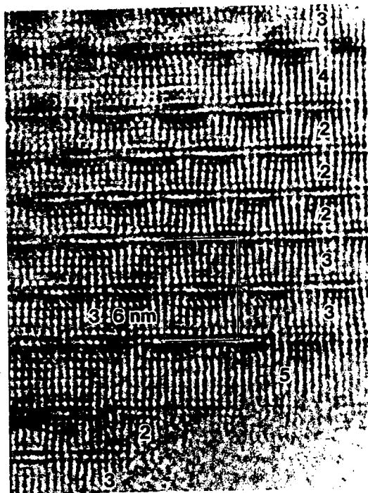
Fig.6 A HRTEM image of \text{Bi}_2(\text{Sr}, \text{Ca})_4\text{Cu}_3\text{O}_y showing the frequent occurrence of intergrowth.
