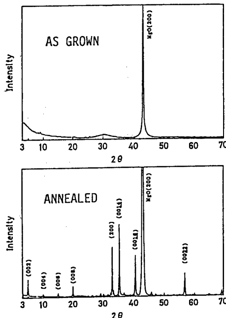
Fig.11 X-ray diffraction of TlBaCaCuO thin film
