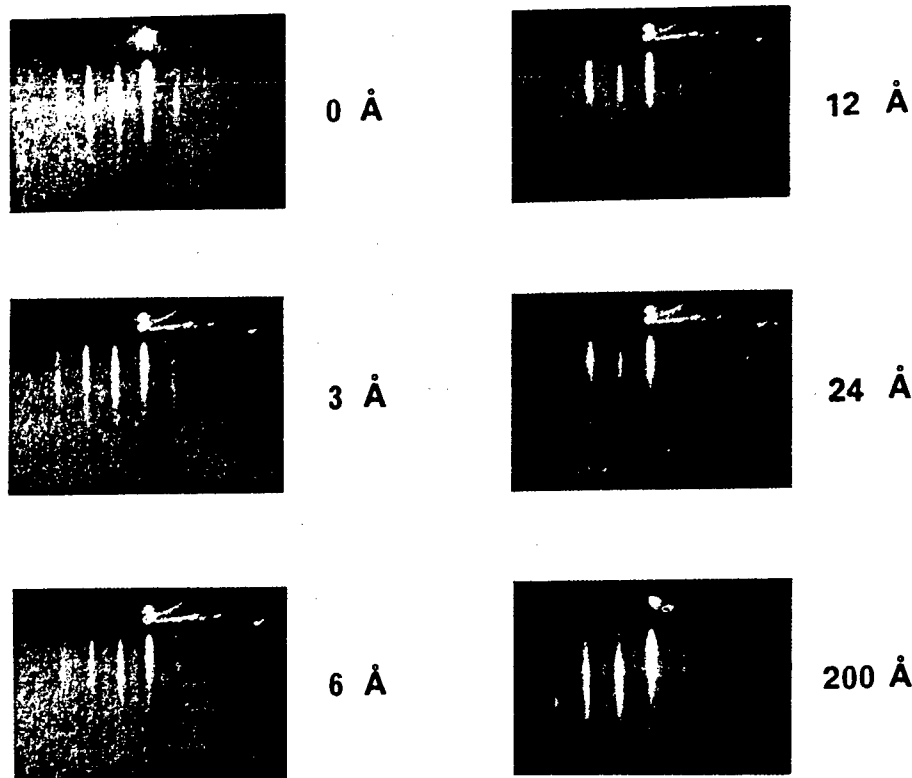
Fig. 2 In-situ RHEED patterns observed during growth of YBCO on SrTiO 3 (100)
