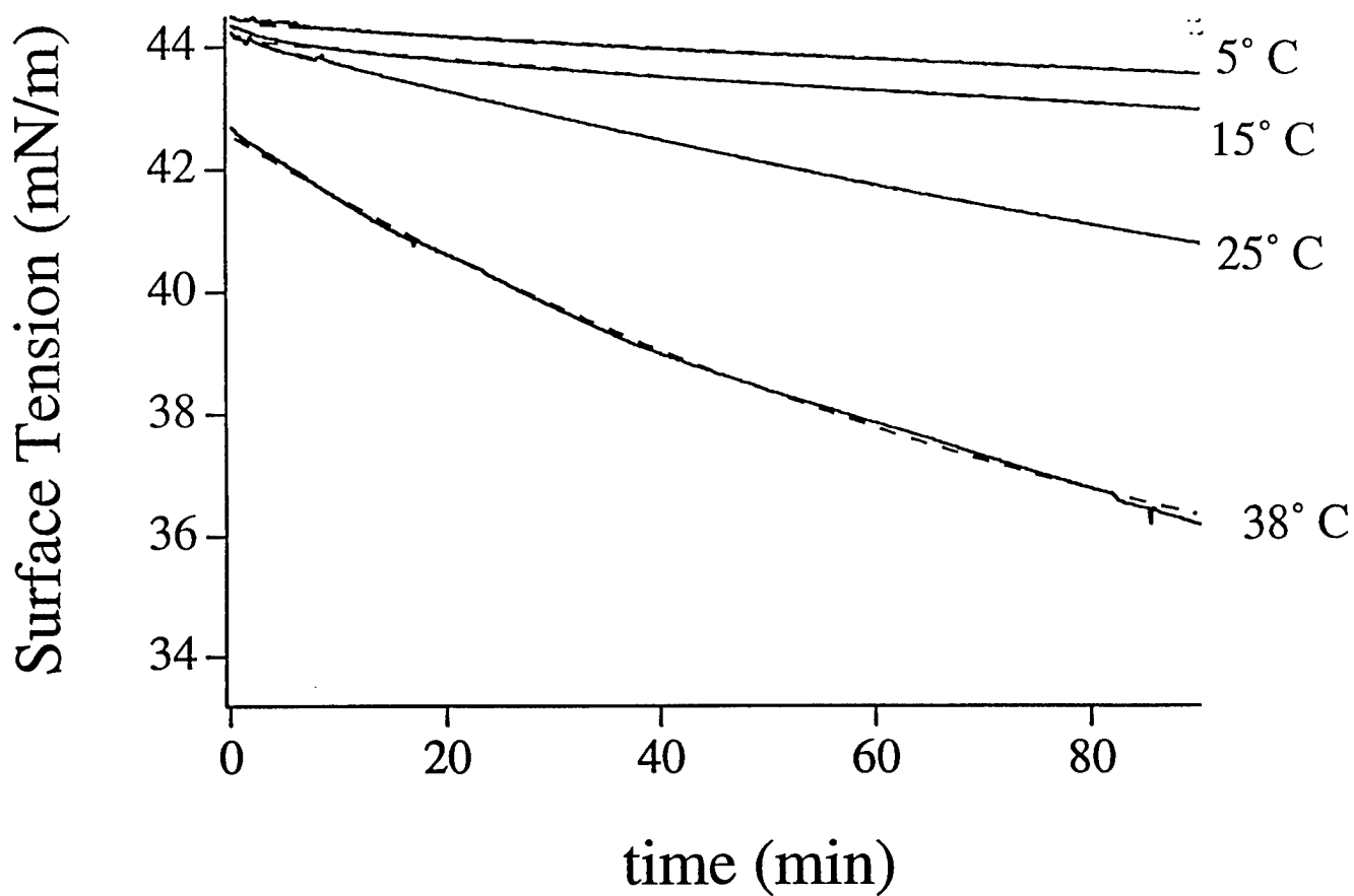
DLPC (0.5 \mu Molar) v. Temperature
