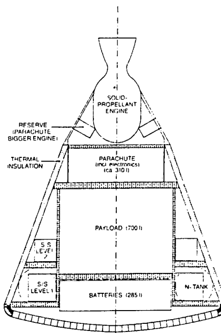
Conceptual design of Space Courier
