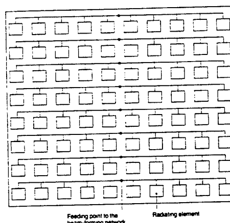
Front view of a microstrip antenna panel
