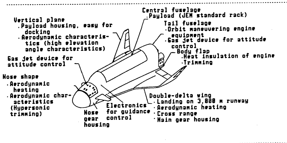
Figure 2. Configuration of HOPE (draft)
