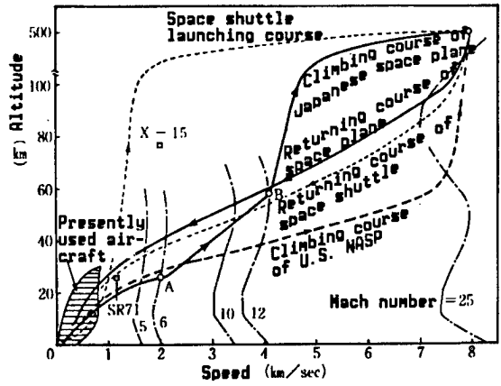
Figure 3. Typical Space Plane Flight Paths
