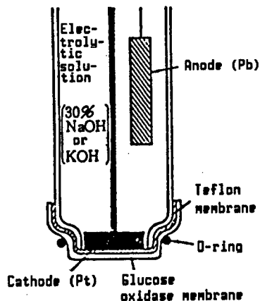
Figure 6. Glucose Sensor
