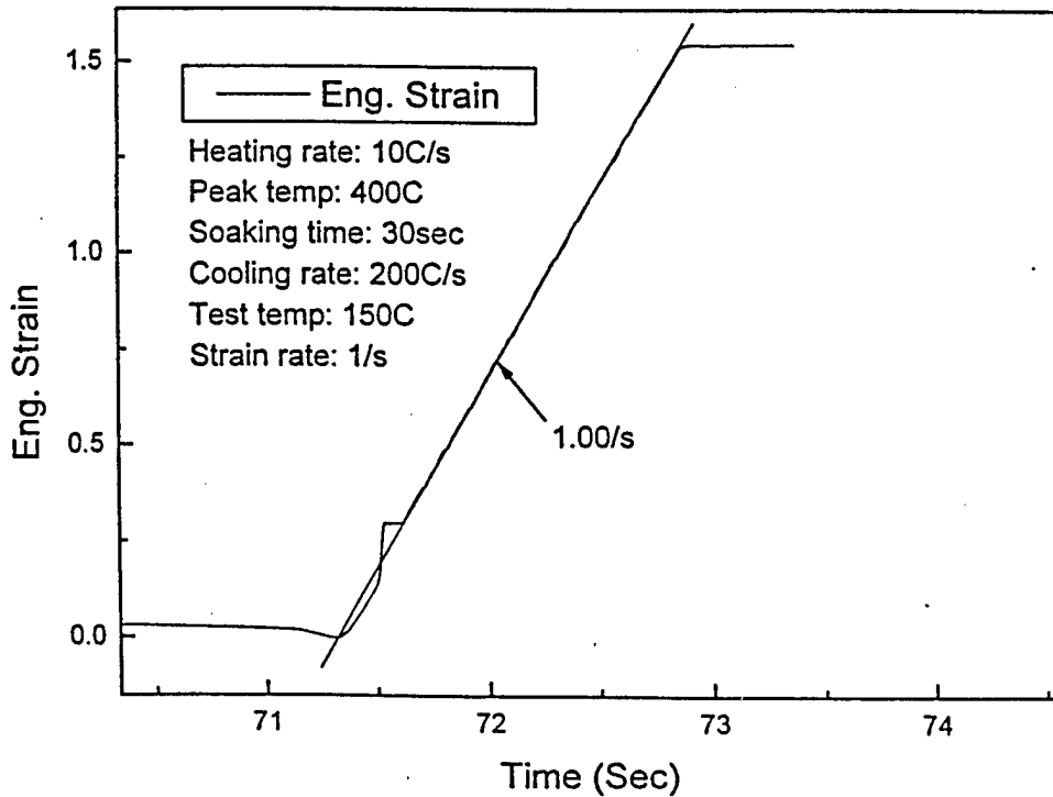
Figure 5 Gleeble Engineering Stress - Strain Curve for Aluminum Alloy 7050
