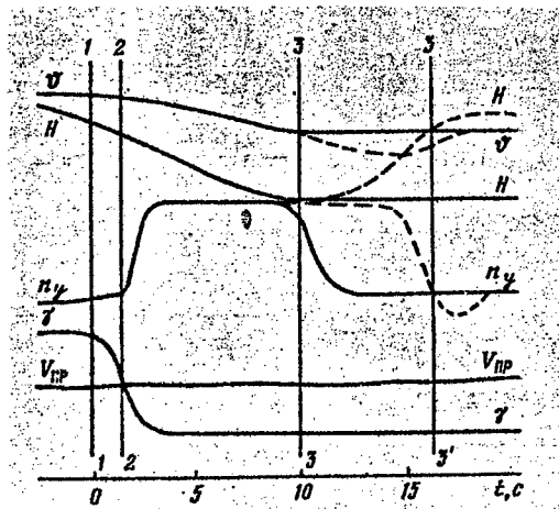
Figure 4. Flight recorder record of flight parameters during aircraft pullout from a descending maneuver by automatic control system
