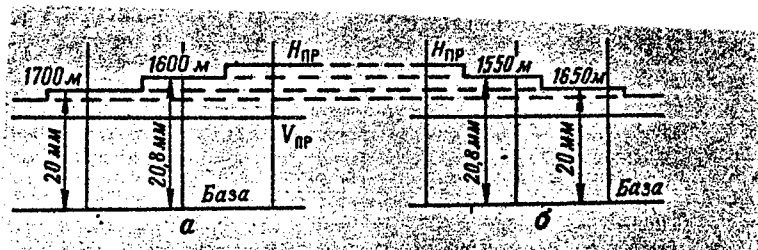
Figure 2. SARPP-12 system altitude record: a) during descent; b) during climb
