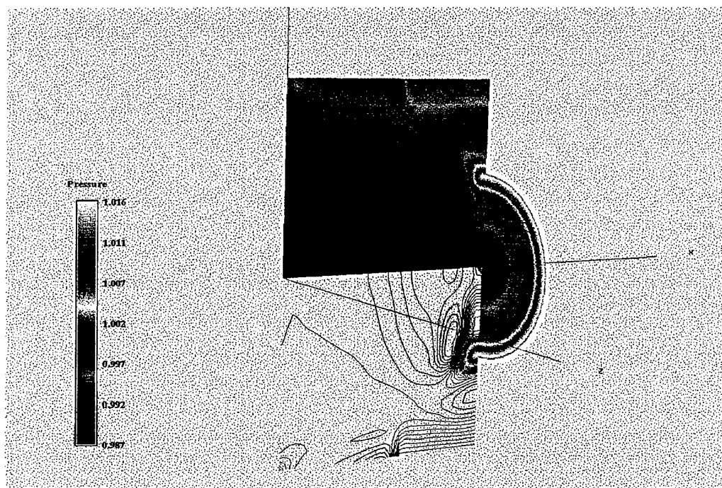
Figure 4a. \frac{P}{P_o} Distribution / 266 Hz Disk Frequency
