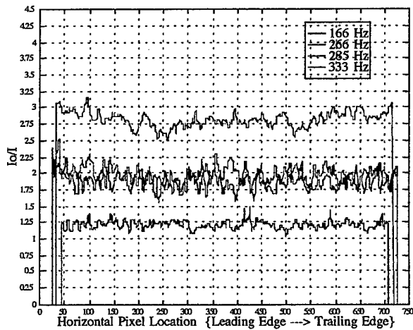
Figure 23c. Horizontal I_0/I Distribution at Vertical Station Y = 83\% Disk Radius
