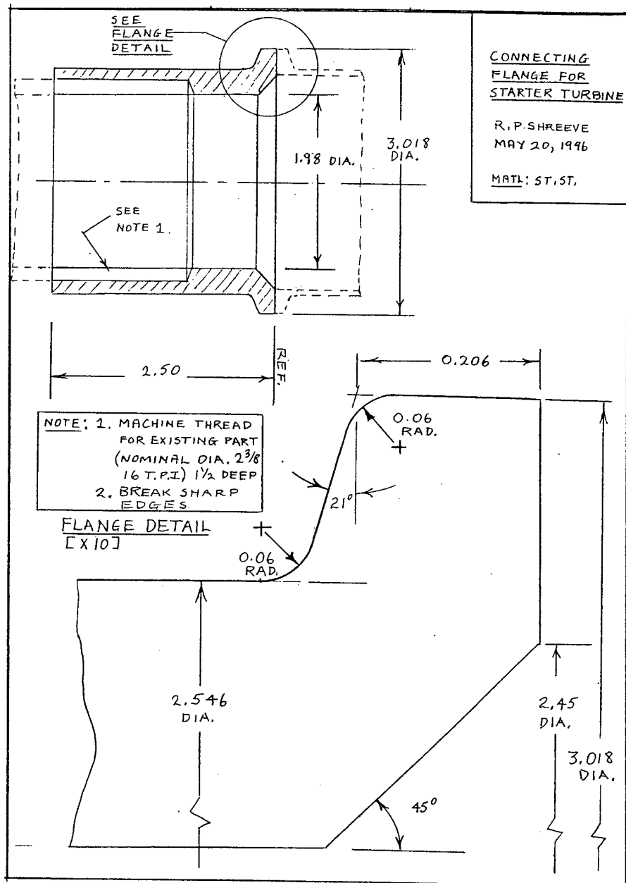
Figure B5. Turbine Connecting Flange Detailed Drawing
