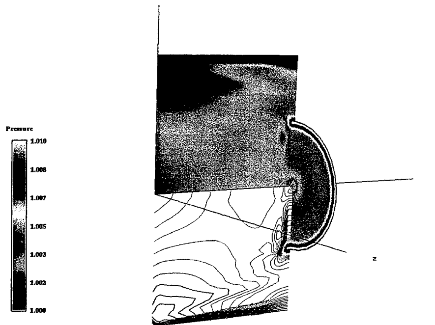
Figure 3a. \frac{P}{P_o} Distribution at 166 Hz Disk Frequency
