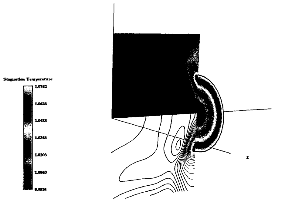
Figure 3b. \frac{T_t}{T_{to}} Distribution at 166 Hz Disk Frequency
