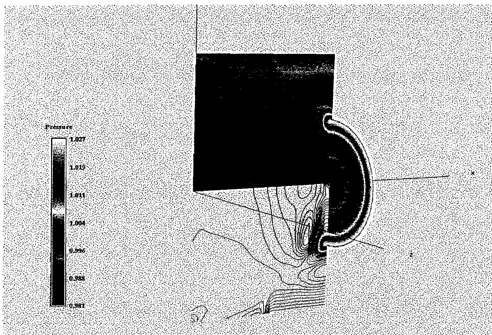
Figure 6a. \frac{P}{P_o} Distribution / 333 Hz Disk Frequency
