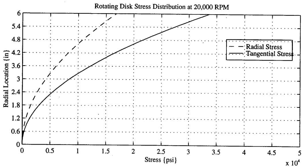
Figure E1. Disk-Rotor Stress Distributions
