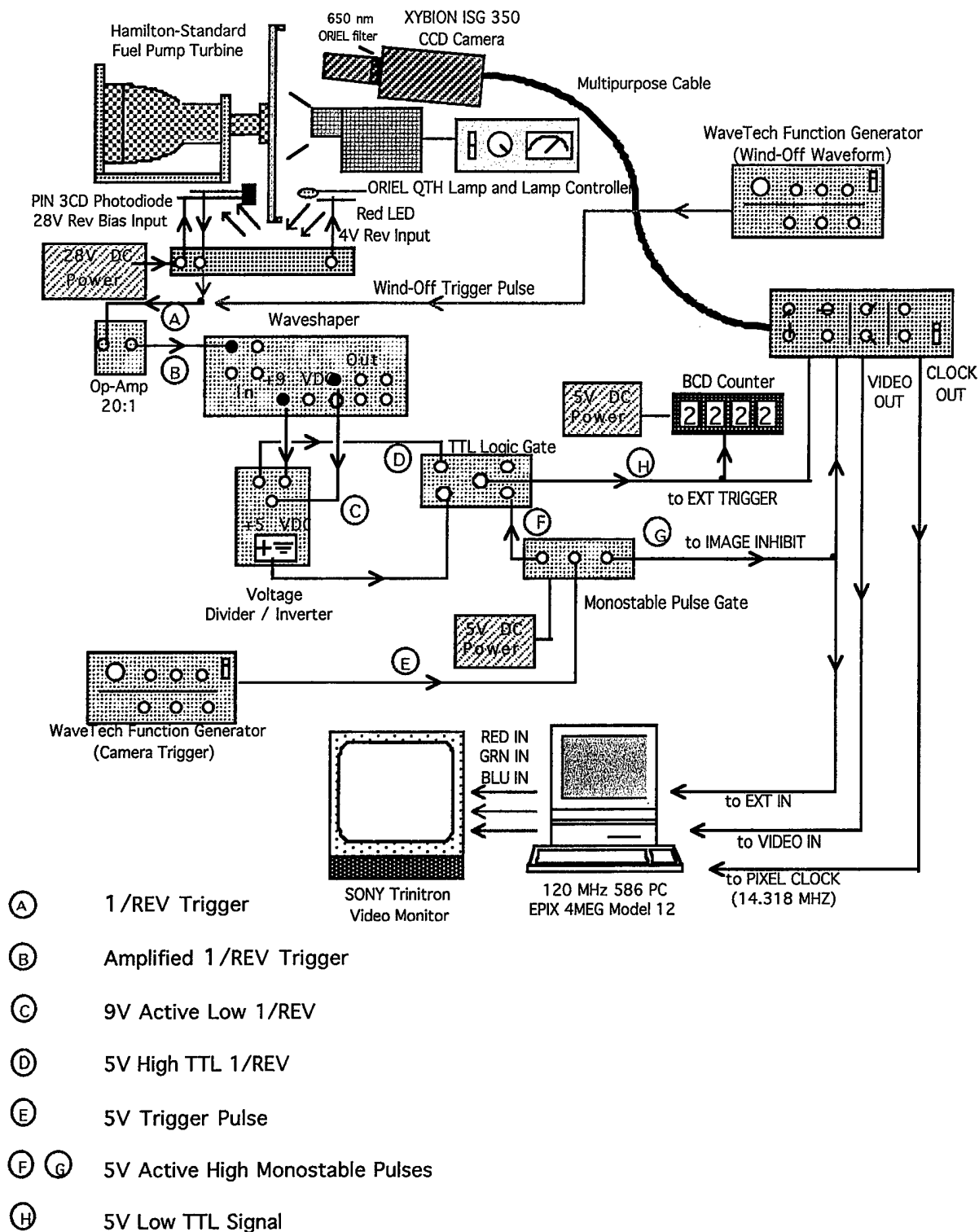
Figure 7. PSP Experimental Setup
