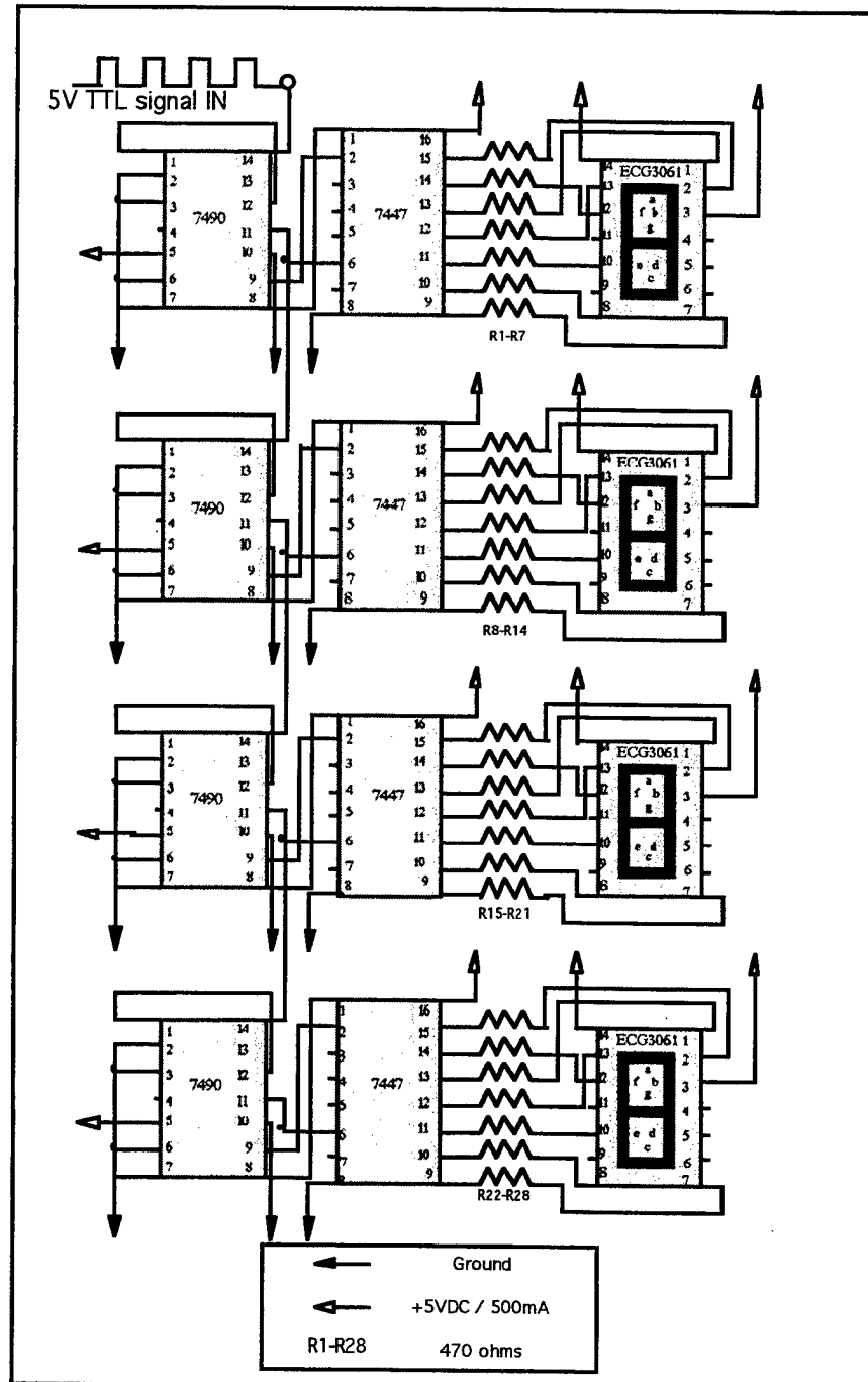
Figure C1. BCD Counter Circuit
