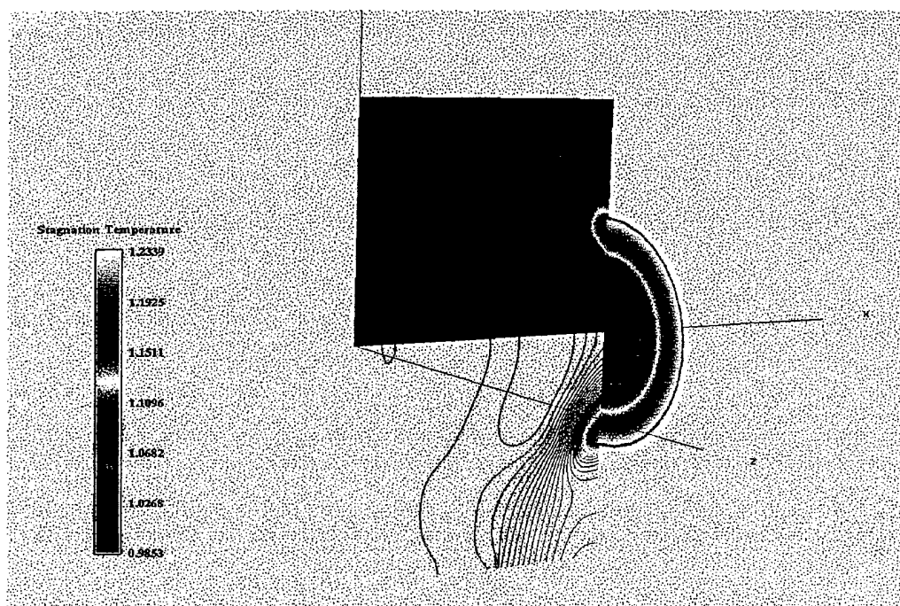
Figure 5b. \frac{T_t}{T_{t0}} Distribution / 285 Hz Disk Frequency
