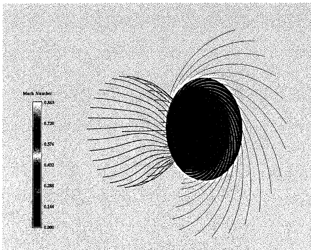
Figure 2. Streamline Trace of Flow About Rotating Disk 333 Hz / Case 4
