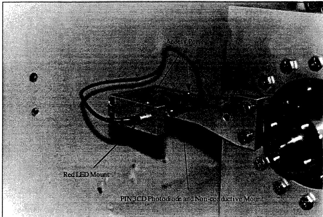
Figure 14. LED / Photodiode Pair and Mounting Bracket
