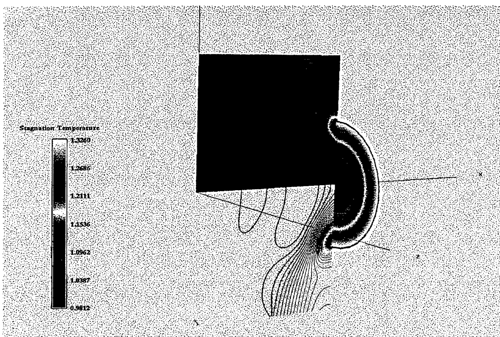
Figure 6b. \frac{T_t}{T_{to}} Distribution / 333 Hz Disk Frequency
