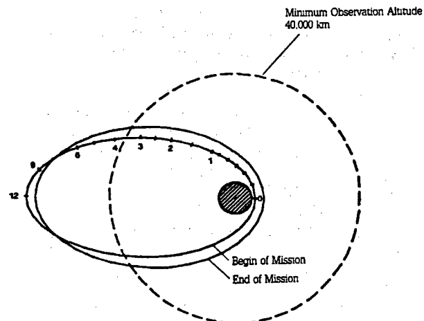
Geometry of the 24 hour highly eccentric orbit (inclination 60°)
