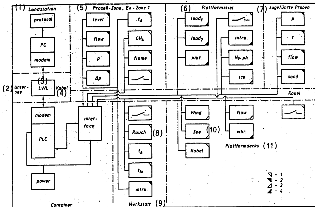
Figure 3. Integrated Optoelectronic Safety System for the Open Sea (1 Fire Prevention, 2 Gas Detection, 3 Environmental Monitor, 4 Platform Monitor: intru. = intrusion, Hy.ph. = hydrophone)
