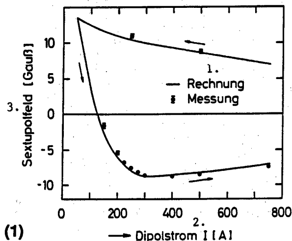
Figure 1. The sextupole field in a superconducting dipole magnet for increasing and decreasing current. The lower curve is used for the injection of the protons at 246 A.
