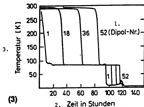
Figure 3. The cooling procedure of the first HERA octant consisting of 52 superconducting dipoles and 26 superconducting quadrupoles. The diagram shows the temperature profile in four dipoles.
