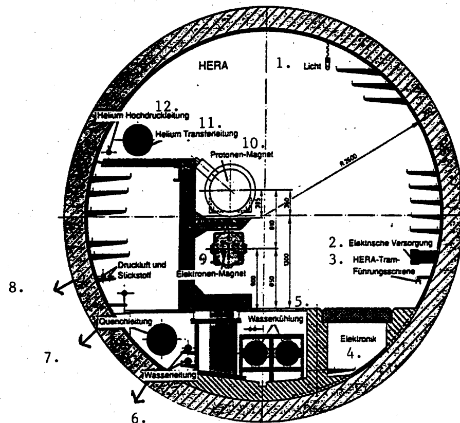
One of the arcs of the HERA tunnel where the particles are bent by magnets. The proton ring is mounted on top of the electronic ring
