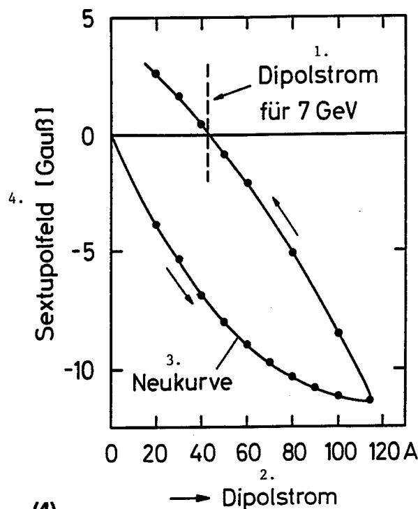
Figure 4. The diagram shows a special running-in procedure of the superconducting proton magnets during the first octant test, before 7 GeV positrons were injected into this 700 m long section. The disturbing sextupole field vanished if the upper curve is used
