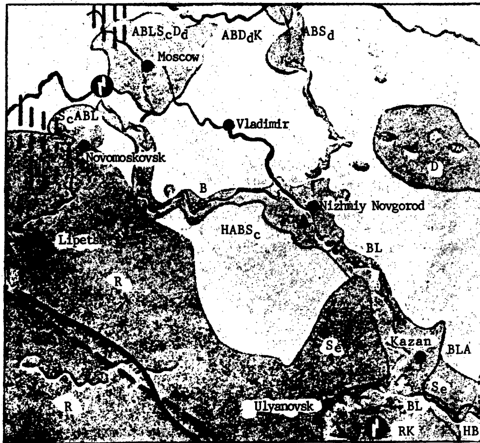
Excerpt from the Ecological Map of the USSR (Scale 1:8 000 000)
