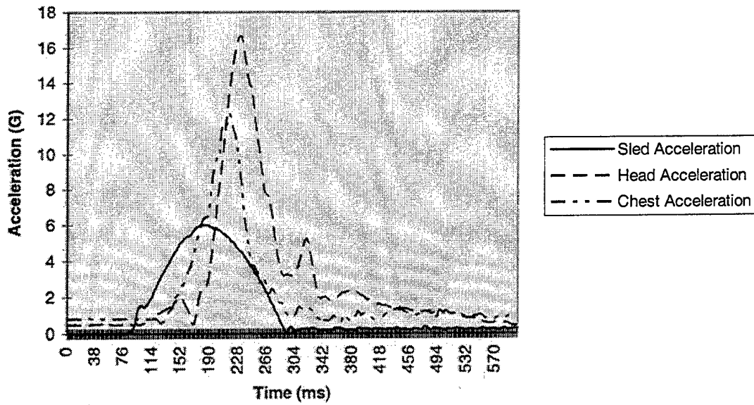
Figure 1. Head and Chest Accelerations from Test 4283 (6G Peak, 210ms Duration)
