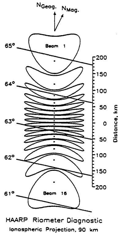
Figure 4. Ionospheric projection of the prototype 16-element HAARP riometer installed at Gakona, Alaska. The antenna array is phased only in the meridional direction, with the 16 beams numbered 1 (most northern) through 16 (most southern). Lines of constant magnetic invariant latitude 61° to 65° are indicated.
