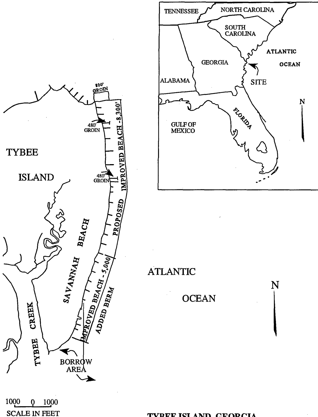
TYBEE ISLAND, GEORGIA BEACH EROSION CONTROL AND HURRICANE PROTECTION PLAN OF IMPROVEMENT
