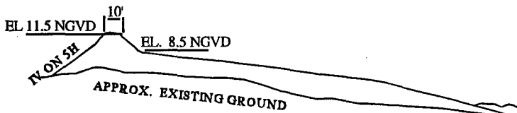
TYPICAL DUNE SECTION
