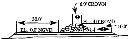
TYPICAL JETTY SECTION
