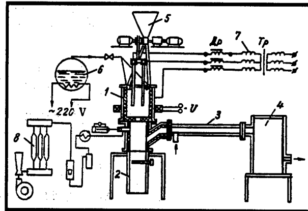
Figure 1. Experimental Engineering Unit for Plasma Conversion of Coal
