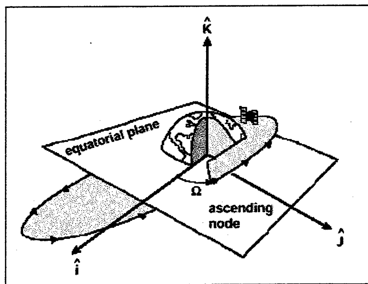
Figure 4. Satellite Coordinate Systems, From Ref. [7].
