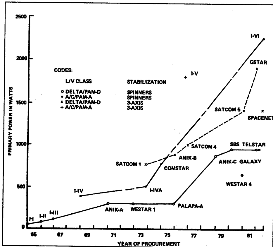
Figure 16. Satellite Power , From Ref. [11]
