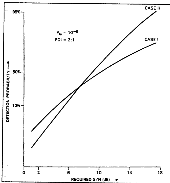
Figure 14. Signal to Noise vs. Detection Probability, From Ref. [6].
