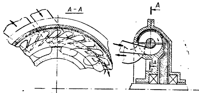
Figure 3. Diagram of a vortex turbine
