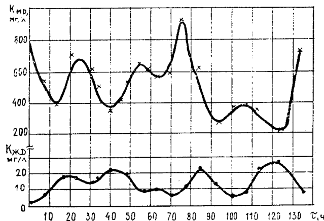
Figure 2. Change in the concentrations of introduced MD ( K_{md} ) substance and the iron-bearing substances ( K_{zhd} ) depending on the duration of the working period (according to the results of atom-absorption ultimate analysis of the fuel).
