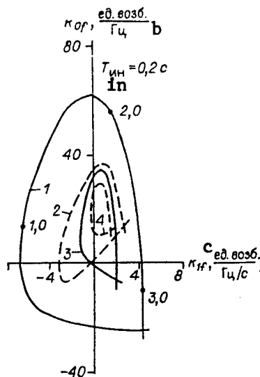
Figure 1. Using an IN [inductive energy storage unit] to suppress synchronous machine oscillations
