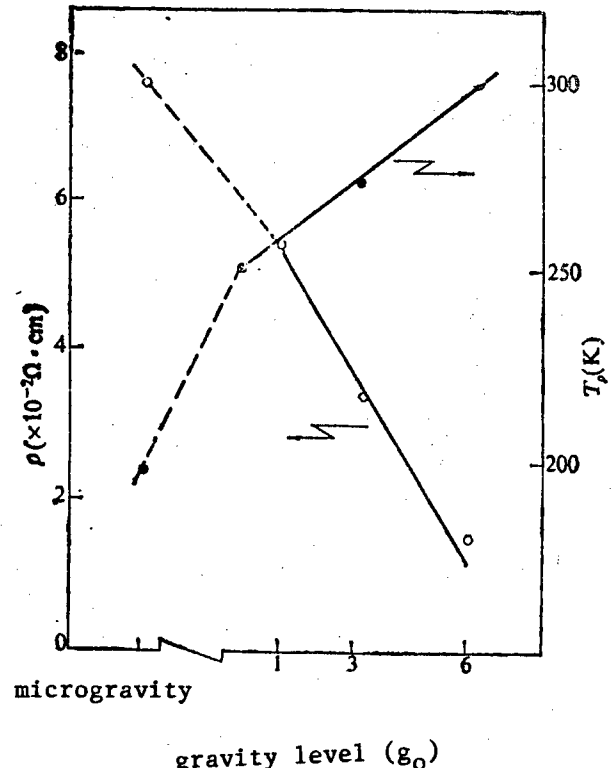
Figure 2. Hall Coefficient Sign-Change Temperature T_R vs. Environmental Gravity g During Preparation
