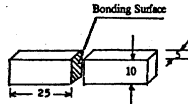
Figure 1. Diffusion Bonding Specimen and Its Size
