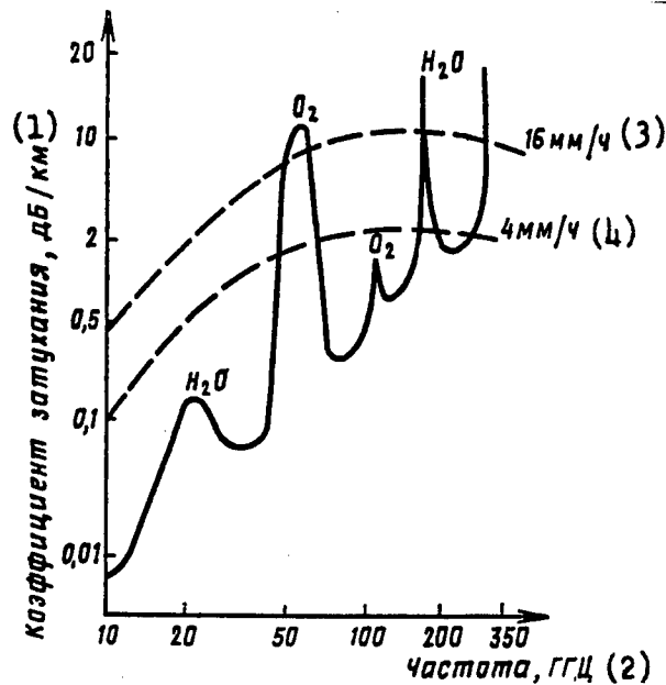
Figure 1. Frequency Characteristics of the Specific Loss of Radio Waves in the Transparent Atmosphere (solid line) and in the Presence of Precipitation (dashed line)
