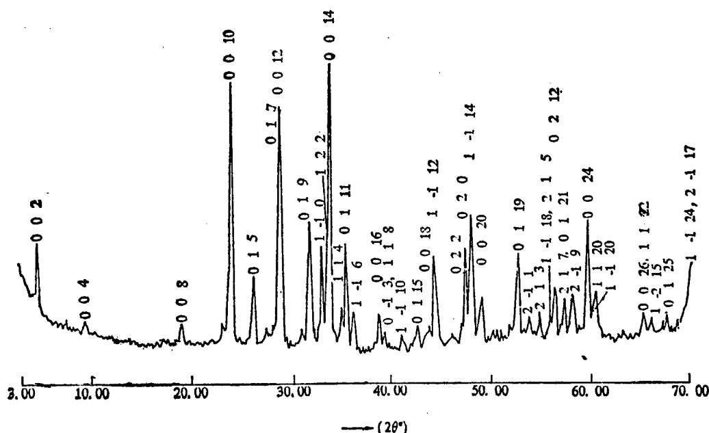
Figure 2. X-Ray Powder Diffraction Pattern of (\text{Pb, Bi})_2\text{Sr}_2\text{Ca}_2\text{Cu}_3\text{O}_y ( \text{CuK} ); reflection is labeled as a monoclinic system and angles specified are 2^\circ .
