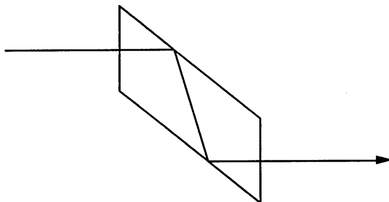
Figure 3-16 Fresnel rhomb achromatic retarder.
