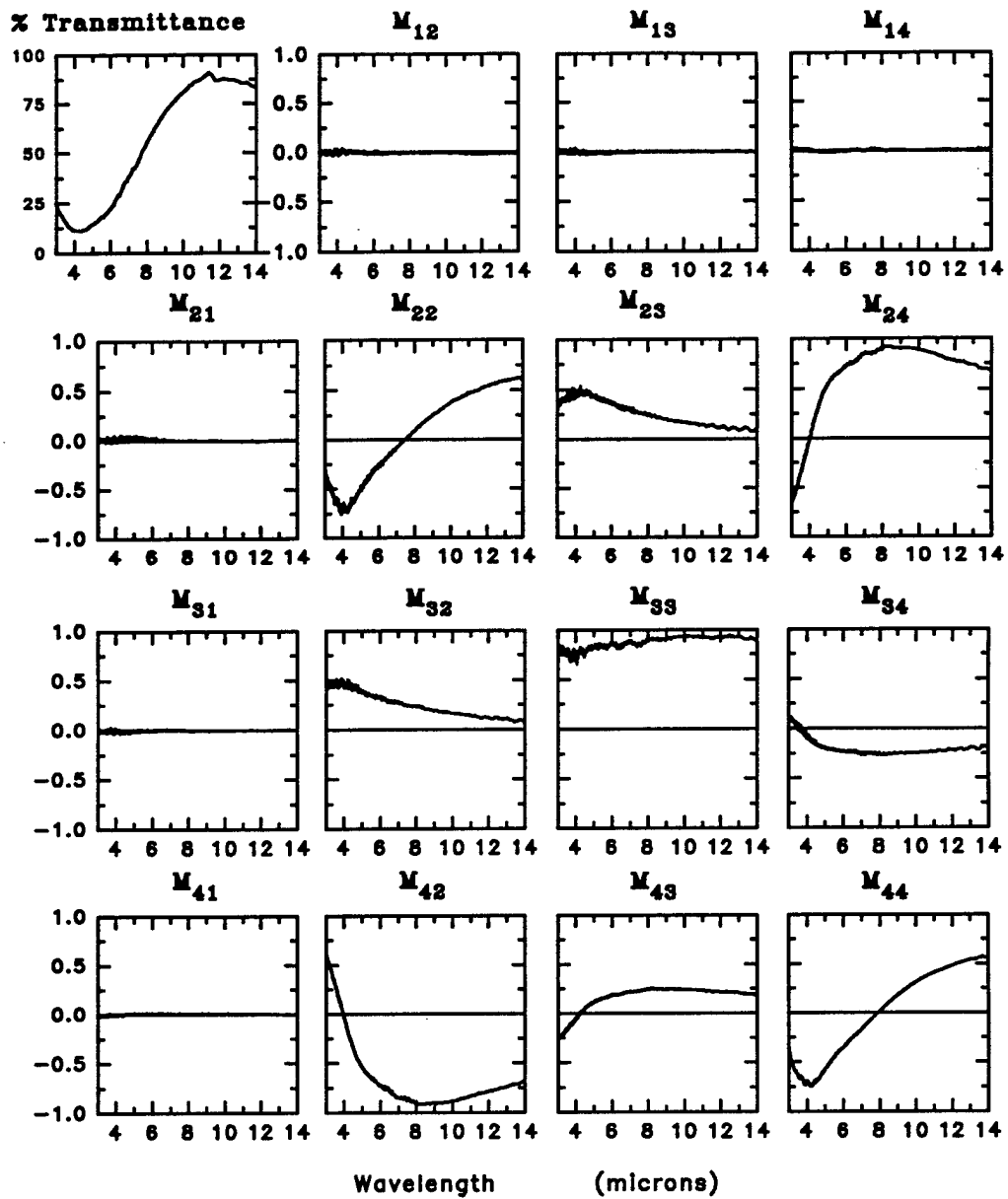
Figure 7-7 Mueller matrix of CdTe modulator with an applied voltage of 1800 volts.
