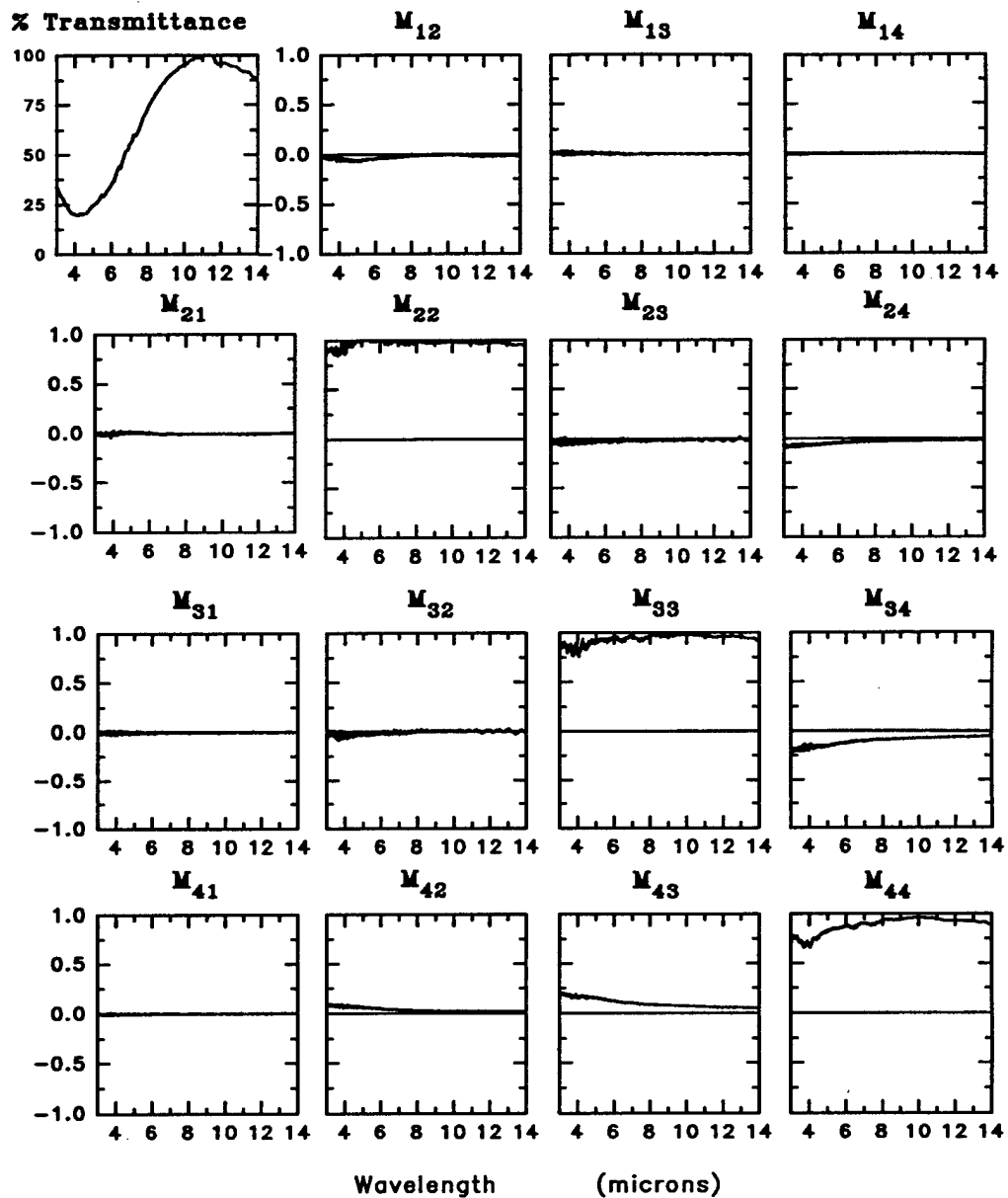
Figure 7-3 Mueller matrix of CdTe modulator with no applied voltage.
