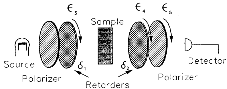
Figure 6-2: The dual rotating retarder polarimeter with retardance and orientation systematic errors.
