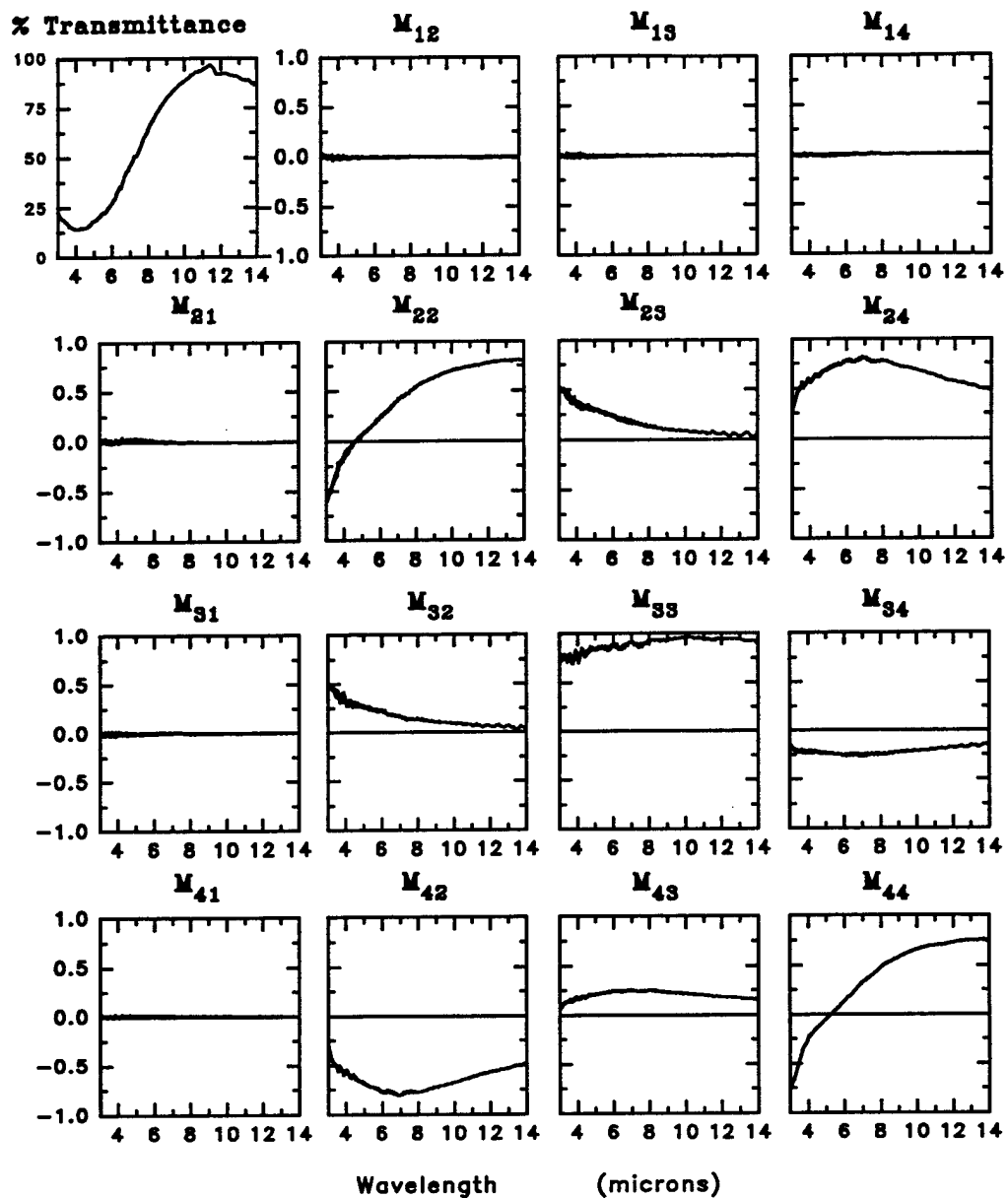
Figure 7-6 Mueller matrix of CdTe modulator with an applied voltage of 1200 volts.
