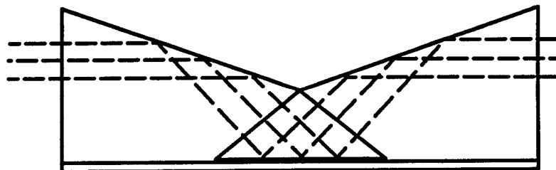
Figure 3-17 Modified Fresnel rhomb achromatic retarder.
