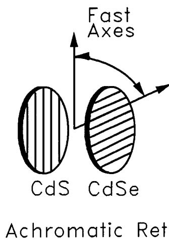
Figure 4-3: The configuration of the achromatic retarder. The angle between the fast axes of the two plates is ideally 90°.
