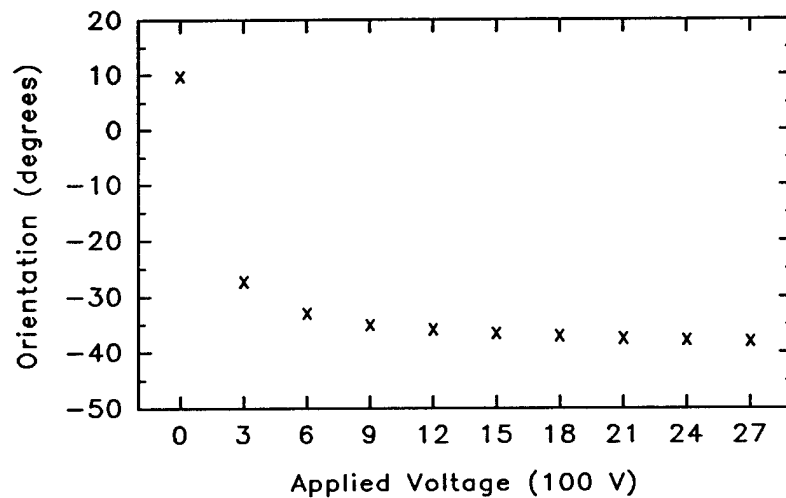
Figure 7-15 Orientation of fast axis as a function of voltage at 10.6 \mu\text{m} .
