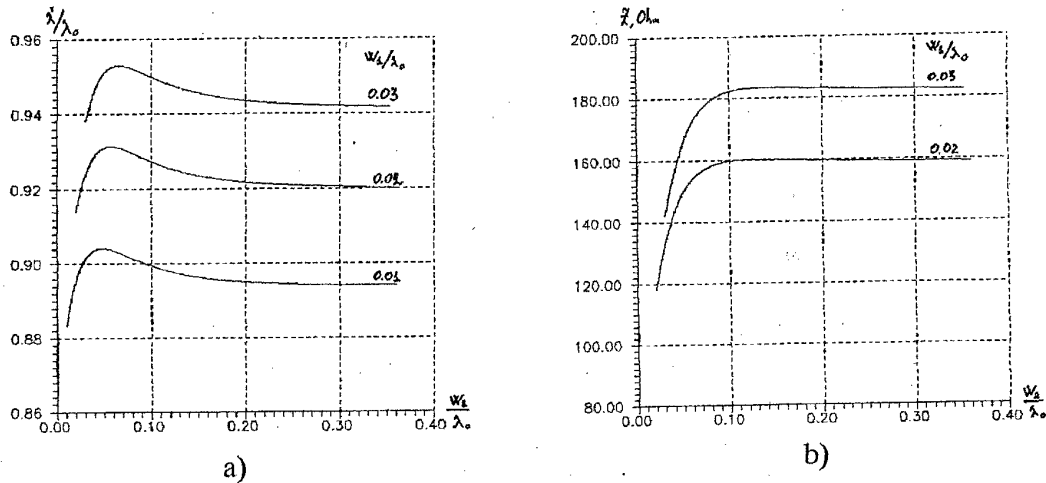
Fig. 9 Normalized wavelength (a) and characteristic impedance (b) of symmetric GDSW with different slot widths versus normalized w_2 : \epsilon_r = 2.22 ; d = 0.254 \text{ mm} (see fig. 2b); h_1 = h_2 = 3.429 \text{ mm} ; waveguide = WR(28)
