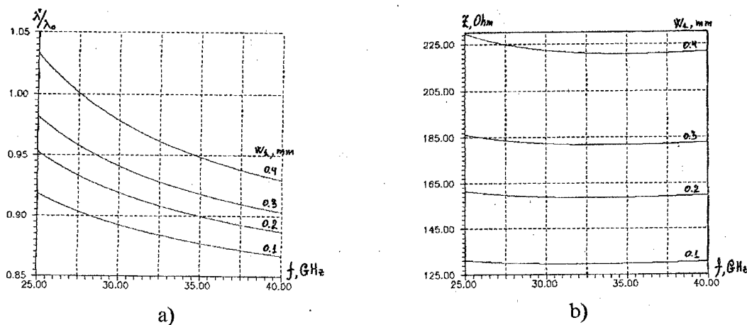
Fig. 5 Normalized guide wavelength \lambda'/\lambda_0 (a) and characteristic impedance Z (b) versus frequency of unilateral fin-line:
