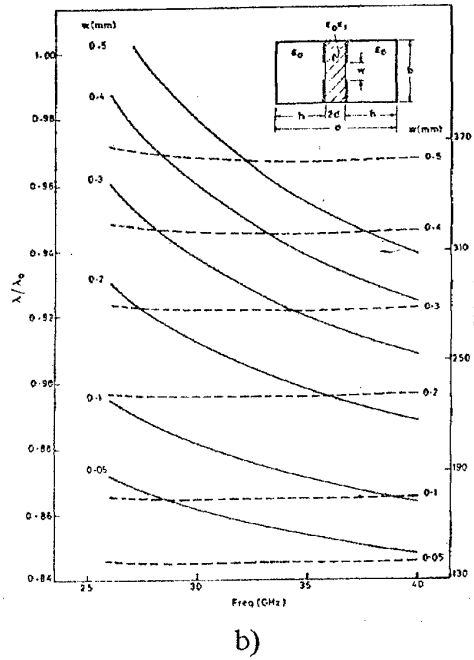
Fig. 6 Normalized guide wavelength \lambda'/\lambda_0 (a) versus frequency of bilateral fin-line and analog from [8] (b):
