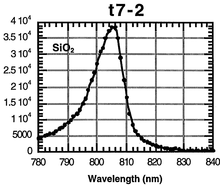
Figure 6.3c Group 3: 12nm relative shift is achieved.
