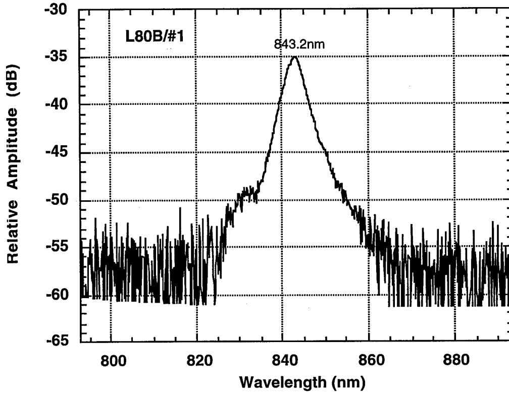
Figure 6.5 The spontaneous emission spectrum of #1 under pumping current just below threshold current on the SrF2 section.
