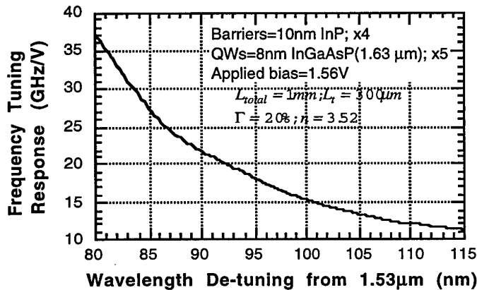
Figure 8.6 Frequency tuning response spectrum for 300µm tuning section length in a 1mm long two-section laser for 1.56V applied reverse bias.
