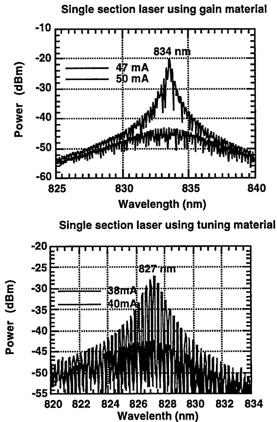
Figure 7.7. Exciton peak de-tuning between gain and tuning section.
