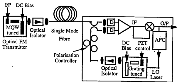
Fig. 4. Experimental optical FMCD link.
