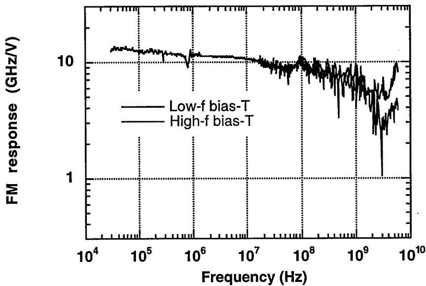
Figure 7.13. FM response of air-bridged laser, with 47 Ω terminating impedance.
