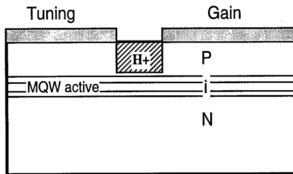
Figure 4.1 H + implantation as the isolation scheme: implantation depth must be above the waveguide in order not to stop the device from lasing.
