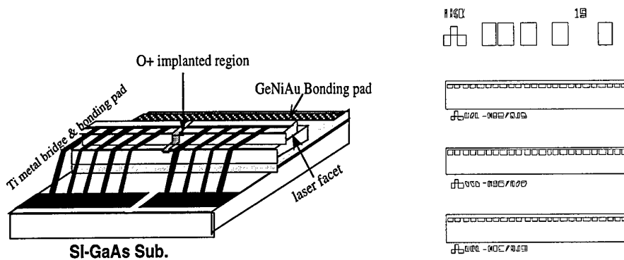
Figure 5.1 Schematic diagram of air-bridged two-section tunable laser and its top contact metalisation mask.
