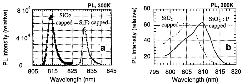
Figure 6.1 Band gap shifting experimental results: (a) capped with \text{SiO}_2 or \text{SrF}_2 ; (b) capped with \text{SiO}_2 or \text{SiO}_2:\text{P} ; all samples were annealed at 900^\circ\text{C} for 30 seconds.
