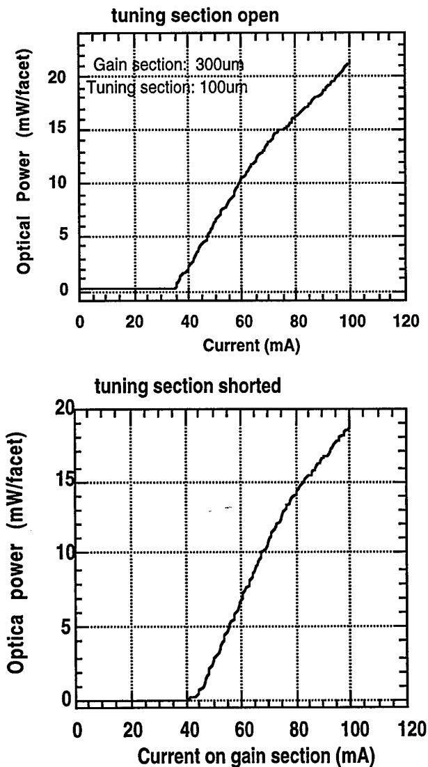
Figure 7.3 L-I plots for air-bridged laser
