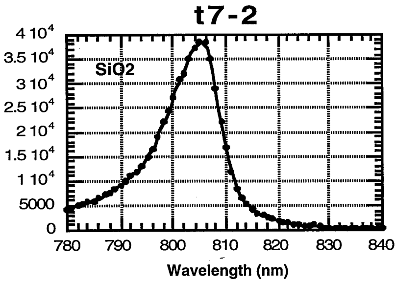
Figure 6.2c Group 3, roughly 1nm shift obtained.
