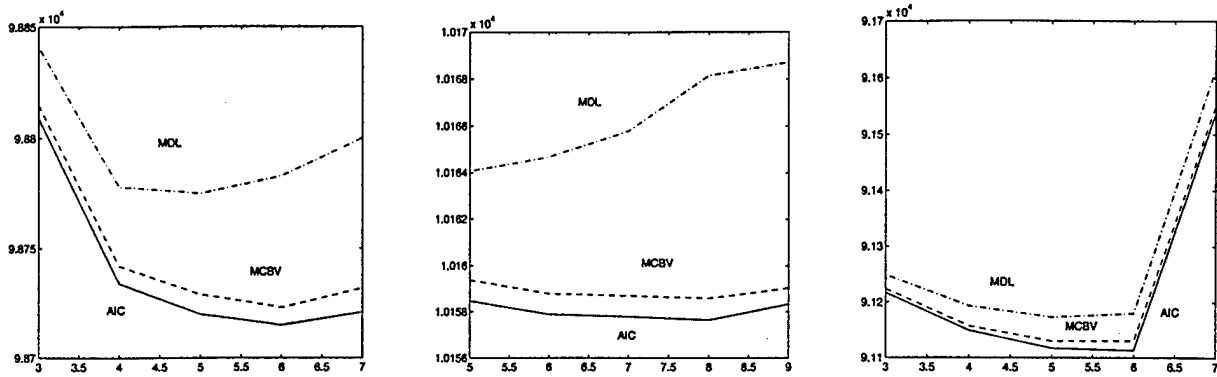
Figure 7: Results of model selection for slice 1-3 ( K_0=6,8,6 , left to right).
