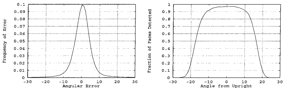
Figure 6: Left: Frequency of errors in the router network with respect to the angular error (in degrees). Right: Fraction of faces that are detected by the detector networks, as a function of the angle of the face from upright.
