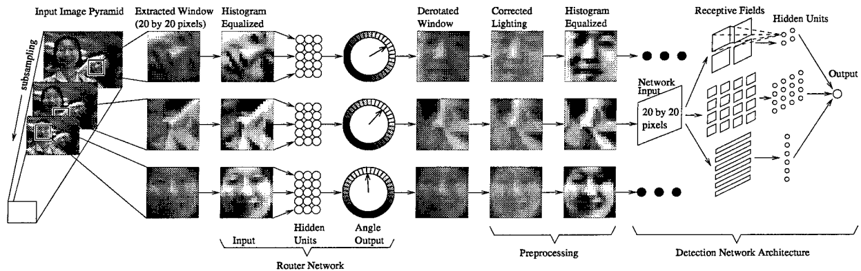
Figure 2: Overview of the algorithm.
