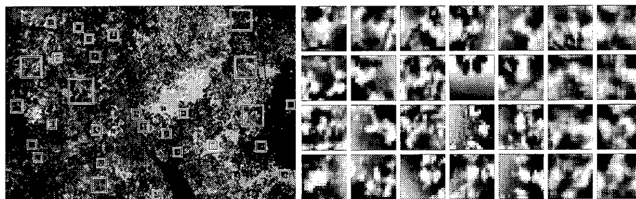
Figure 5: Left: The partially-trained system is applied to images of scenery which do not contain faces. Right: Any regions in the image detected as faces are errors, which can be added into the set of negative training examples.
