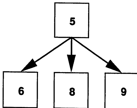
Precedence Graph
