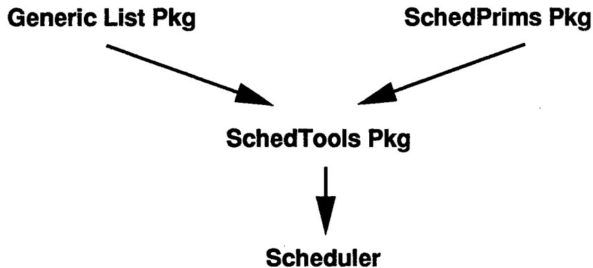
Library Dependence Structure.
