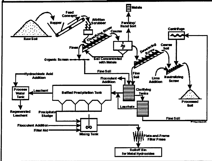
Figure 11. Vendor 2's plant and the hydrochloric acid process.
