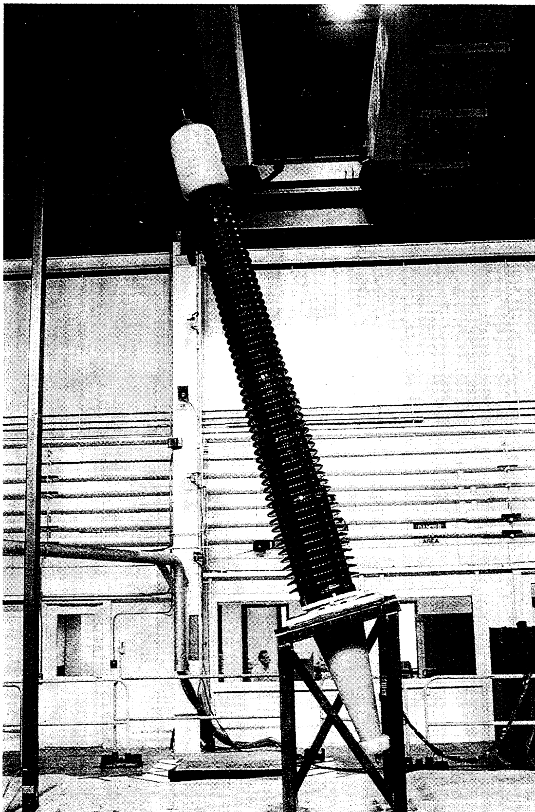
Figure 1. TVA power transformer bushing tested on the USACERL TESS.
