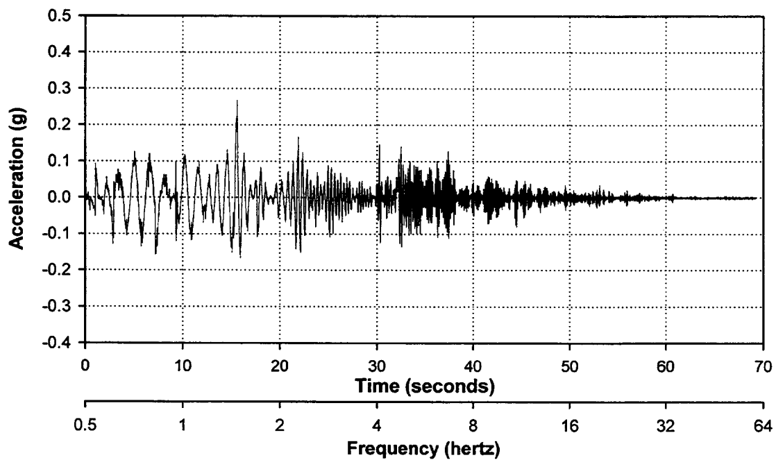
Figure 8a. Achieved lateral acceleration with input motions at 29% of Figure 7a.
