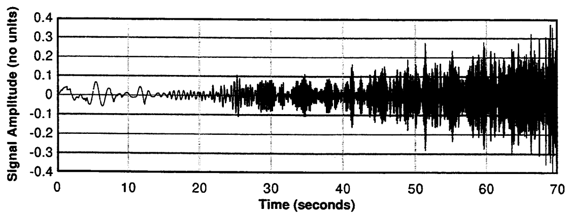
Figure 3a. Generated narrow-band random signal, Ran1.
