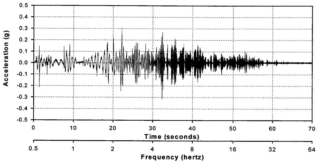
Figure 10b. Achieved longitudinal acceleration, 50% of Figure 7b with 1.2hz HP Filter.
