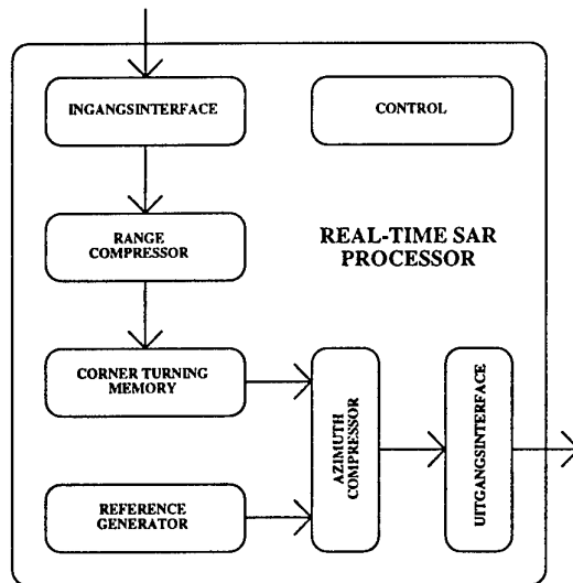
Figuur 2.3: Systeemopzet Real-Time SAR Processor.
