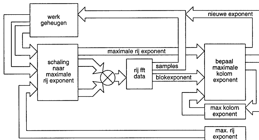
Figuur 3.9: Dataflow in state 6.
