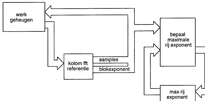
Figuur 3.5: Dataflow in state 2.
