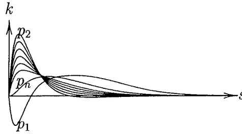
Figure 39. Curvature Plots for Leaving Points at y = 7, 4.712, 3.5, 3, 2.5, 2, 1.5 and 1 .
