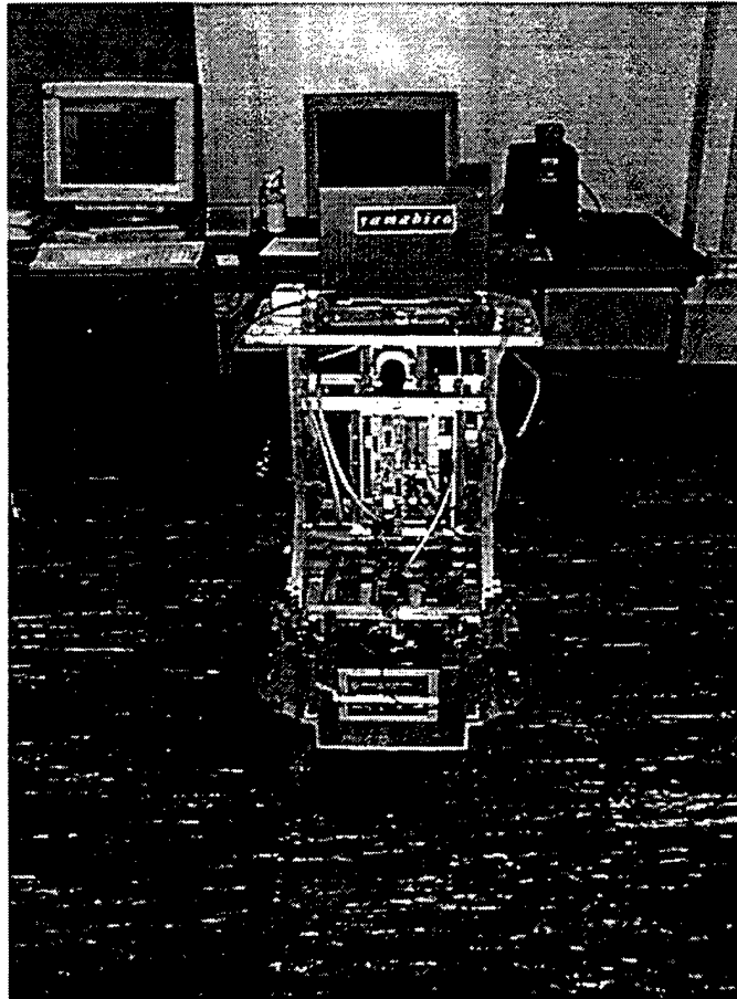
Figure 25. Robot "Yamabico"
