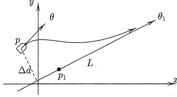
Figure 34. Principle of Path Tracking
