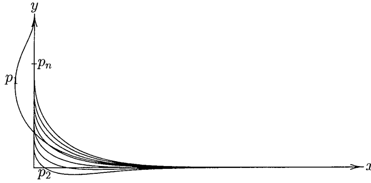
Figure 38. Trajectory for Leaving Points at y = 7, 4.712, 3.5, 3, 2.5, 2, 1.5 and 1 .
