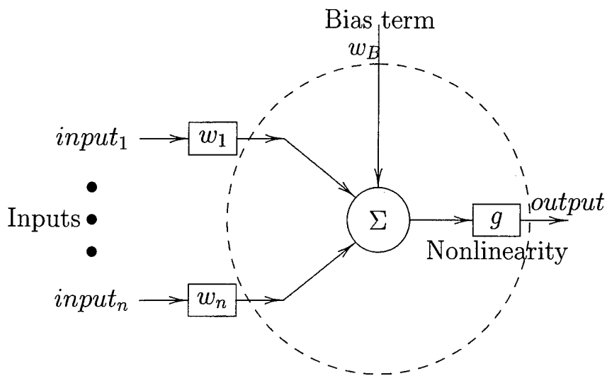
Figure 3. Basic Neuron (Node or PE) Model.
