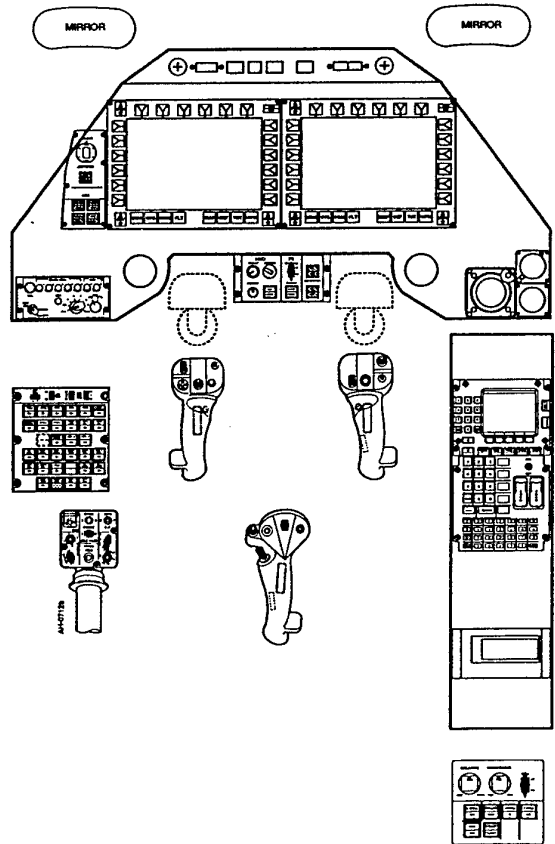
Figure 3 Two-dimensional Layout of Rear Cockpit
